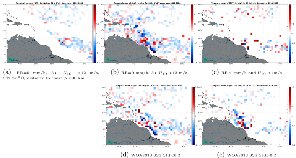
Figure 13: Temporal mean gridded over spatial boxes of size 1^\circ \times 1^\circ of \Delta\text{SSS} (SMOS SSS L3 v332 - 9 Days (CATDS-CPDC) - Surface drifters) for 5 different subdatasets corresponding to:RR=0 mm/h, 3 < U_{10} < 12 m/s, SST >5^\circ\text{C} , distance to coast > 800 km (a), RR=0 mm/h, 3 < U_{10} < 12 m/s (b), RR >1 mm/h and U_{10} < 4 m/s (c), WOA2013 SSS Std <0.2 (d), WOA2013 SSS Std >0.2 (e).
