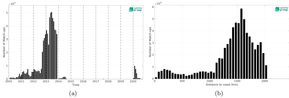
Figure 2: Number of match-ups between Surface drifters and SMOS SSS L3 v332 - 9 Days (CATDS-CPDC) SSS as a function of time (a) and as function of the distance to coast (b) over the Amazon and Orinoco river plumes Pi-MEP region and for the full satellite product period.
