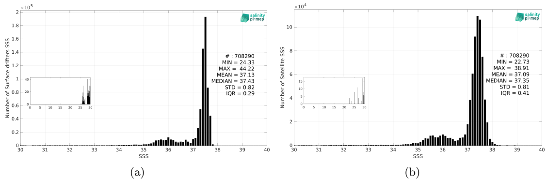
Figure 3: Histograms of SSS from Surface drifters (a) and SMOS SSS L3 v332 - 9 Days (CATDS-CPDC) (b) considering all match-up pairs per bins of 0.1 over the Amazon and Orinoco river plumes Pi-MEP region and for the full satellite product period.
