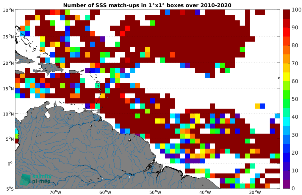
Figure 4: Number of SSS match-ups between Surface drifters SSS and the SMOS SSS L3 v332 - 9 Days (CATDS-CPDC) SSS product for the Amazon and Orinoco river plumes Pi-MEP region over 1^{\circ} \times 1^{\circ} boxes and for the full satellite product period.
