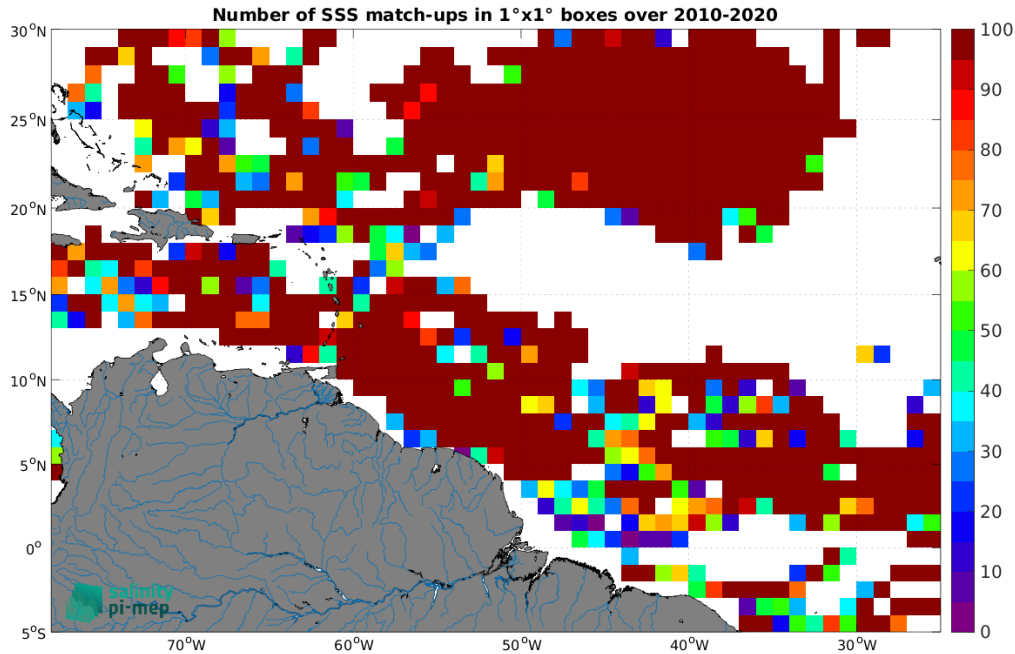
Figure 3: Number of SSS match-ups between Surface drifters SSS and the SMOS SSS L3 v332 - 9 Days (CATDS-CPDC) SSS product for the Amazon and Orinoco river plumes Pi-MEP region over 1^{\circ} \times 1^{\circ} boxes and for the full satellite product period.
