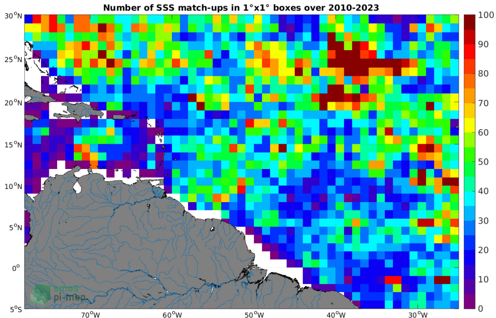
Figure 4: Number of SSS match-ups between Argo SSS and the SMOS SSS L3 v332 - 9 Days (CATDS-CPDC) SSS product for the Amazon and Orinoco river plumes Pi-MEP region over 1^\circ \times 1^\circ boxes and for the full satellite product period.
