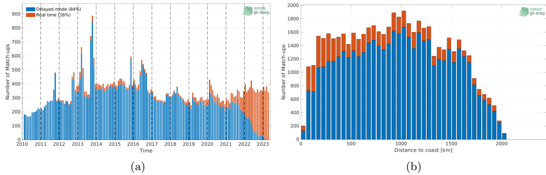
Figure 1: Number of match-ups between Argo and SMOS SSS L3 v332 - 9 Days (CATDS-CPDC) SSS as a function of time (a) and as function of the distance to coast (b) over the Amazon and Orinoco river plumes Pi-MEP region and for the full satellite product period.
