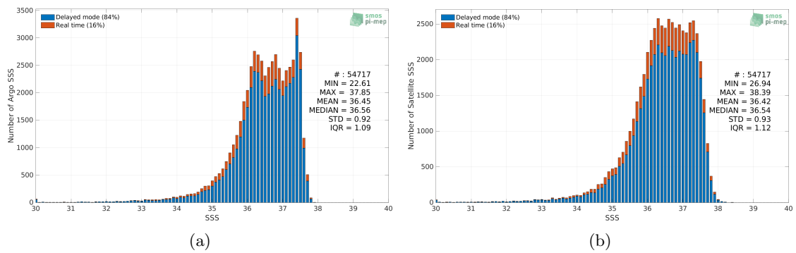
Figure 2: Histograms of SSS from Argo (a) and SMOS SSS L3 v332 - 9 Days (CATDS-CPDC) (b) considering all match-up pairs per bins of 0.1 over the Amazon and Orinoco river plumes Pi-MEP region and for the full satellite product period.
