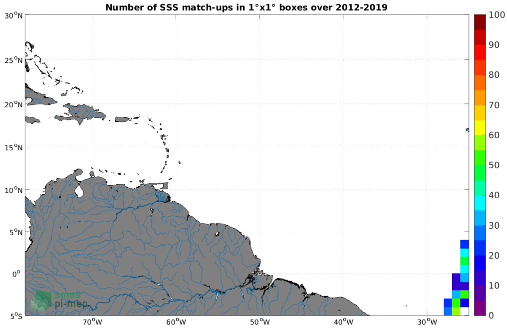
Figure 4: Number of SSS match-ups between TSG (Polarstern) SSS and the SMOS SSS L2Q v330 - 0.25 Deg (CATDS-CPDC) SSS product for the Amazon and Orinoco river plumes Pi-MEP region over 1^\circ \times 1^\circ boxes and for the full satellite product period.
