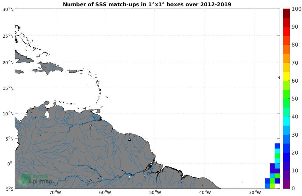
Figure 4: Number of SSS match-ups between TSG (Polarstern) SSS and the SMOS SSS L2Q v330 - 0.25 Deg (CATDS-CPDC) SSS product for the Amazon and Orinoco river plumes Pi-MEP region over 1^{\circ} \times 1^{\circ} boxes and for the full satellite product period.
