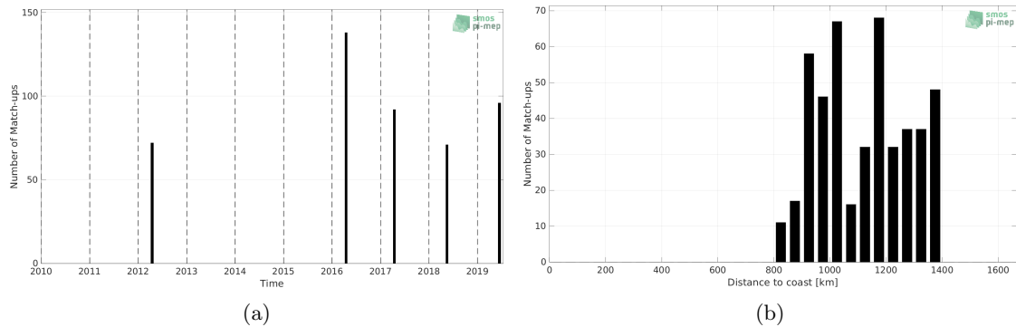
Figure 1: Number of match-ups between TSG (Polarstern) and SMOS SSS L2Q v330 - 0.25 Deg (CATDS-CPDC) SSS as a function of time (a) and as function of the distance to coast (b) over the Amazon and Orinoco river plumes Pi-MEP region and for the full satellite product period.
