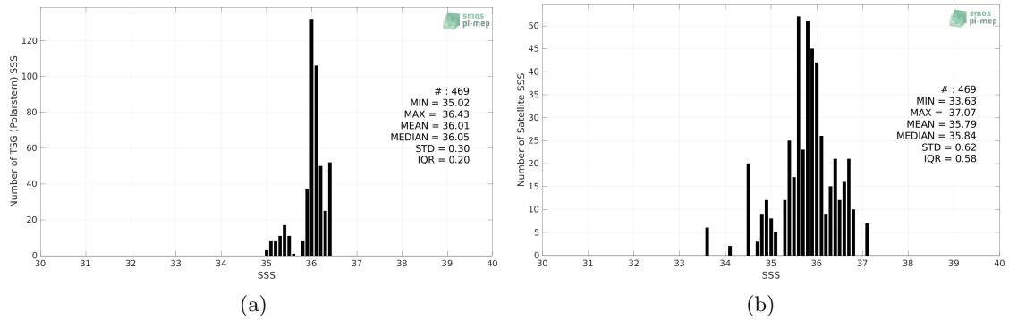
Figure 2: Histograms of SSS from TSG (Polarstern) (a) and SMOS SSS L2Q v330 - 0.25 Deg (CATDS-CPDC) (b) considering all match-up pairs per bins of 0.1 over the Amazon and Orinoco river plumes Pi-MEP region and for the full satellite product period.
