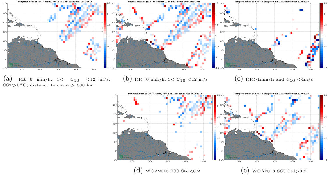
Figure 12: Temporal mean gridded over spatial boxes of size 1^{\circ}\times 1^{\circ} of \Delta\text{SSS} (SMOS SSS L2Q v330 - 0.25 Deg (CATDS-CPDC) - TSG (LEGOS-DM)) for 5 different subdatasets corresponding to: RR=0 mm/h, 3 < U_{10} < 12 m/s, SST >5^{\circ}\text{C} , distance to coast > 800 km (a), RR=0 mm/h, 3 < U_{10} < 12 m/s (b), RR >1 mm/h and U_{10} < 4 m/s (c), WOA2013 SSS Std <0.2 (d), WOA2013 SSS Std >0.2 (e).
