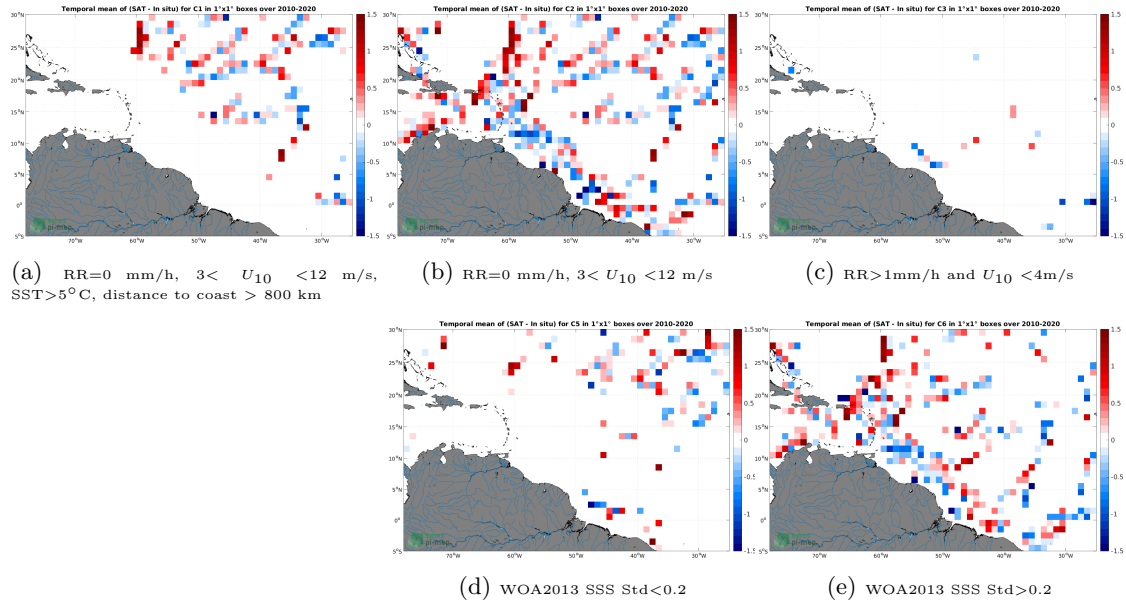
Figure 12: Temporal mean gridded over spatial boxes of size 1^{\circ}\times 1^{\circ} of \Delta SSS (SMOS SSS L2Q v330 - 0.25 Deg (CATDS-CPDC) - TSG (GOSUD-Research-vessel)) for 5 different subdatasets corresponding to:RR=0 mm/h, 3 < U_{10} < 12 m/s, SST >5^{\circ}\text{C} , distance to coast > 800 km (a), RR=0 mm/h, 3 < U_{10} < 12 m/s (b), RR >1 mm/h and U_{10} < 4 m/s (c), WOA2013 SSS Std <0.2 (d), WOA2013 SSS Std >0.2 (e).
