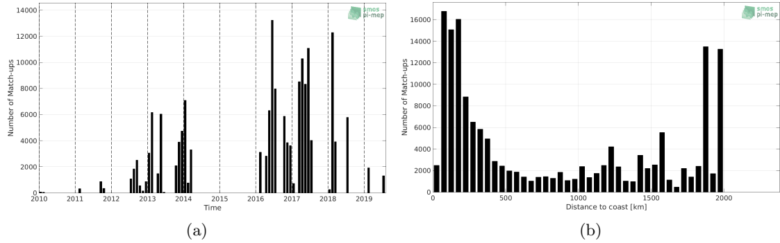
Figure 1: Number of match-ups between TSG (GOSUD-Research-vessel) and SMOS SSS L2Q v330 - 0.25 Deg (CATDS-CPDC) SSS as a function of time (a) and as function of the distance to coast (b) over the Amazon and Orinoco river plumes Pi-MEP region and for the full satellite product period.
