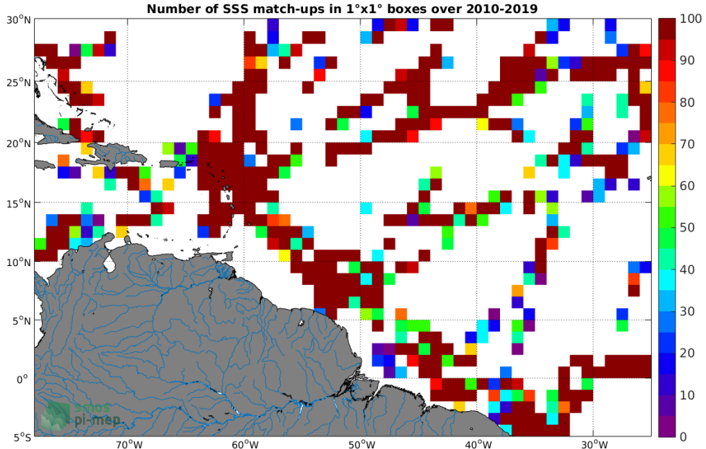
Figure 4: Number of SSS match-ups between TSG (GOSUD-Research-vessel) SSS and the SMOS SSS L2Q v330 - 0.25 Deg (CATDS-CPDC) SSS product for the Amazon and Orinoco river plumes Pi-MEP region over 1^\circ \times 1^\circ boxes and for the full satellite product period.
