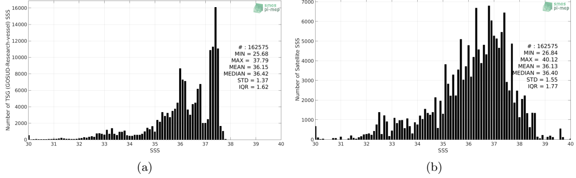
Figure 2: Histograms of SSS from TSG (GOSUD-Research-vessel) (a) and SMOS SSS L2Q v330 - 0.25 Deg (CATDS-CPDC) (b) considering all match-up pairs per bins of 0.1 over the Amazon and Orinoco river plumes Pi-MEP region and for the full satellite product period.
