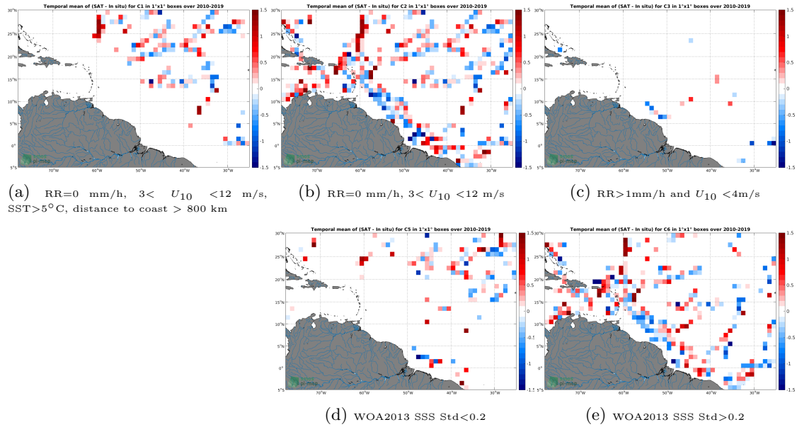
Figure 12: Temporal mean gridded over spatial boxes of size 1^\circ \times 1^\circ of \Delta SSS (SMOS SSS L2Q v330 - 0.25 Deg (CATDS-CPDC) - TSG (GOSUD-Research-vessel)) for 5 different subdatasets corresponding to: RR=0 mm/h, 3 < U_{10} < 12 m/s, SST > 5^\circ\text{C} , distance to coast > 800 km (a), RR=0 mm/h, 3 < U_{10} < 12 m/s (b), RR > 1 mm/h and U_{10} < 4 m/s (c), WOA2013 SSS Std < 0.2 (d), WOA2013 SSS Std > 0.2 (e).
