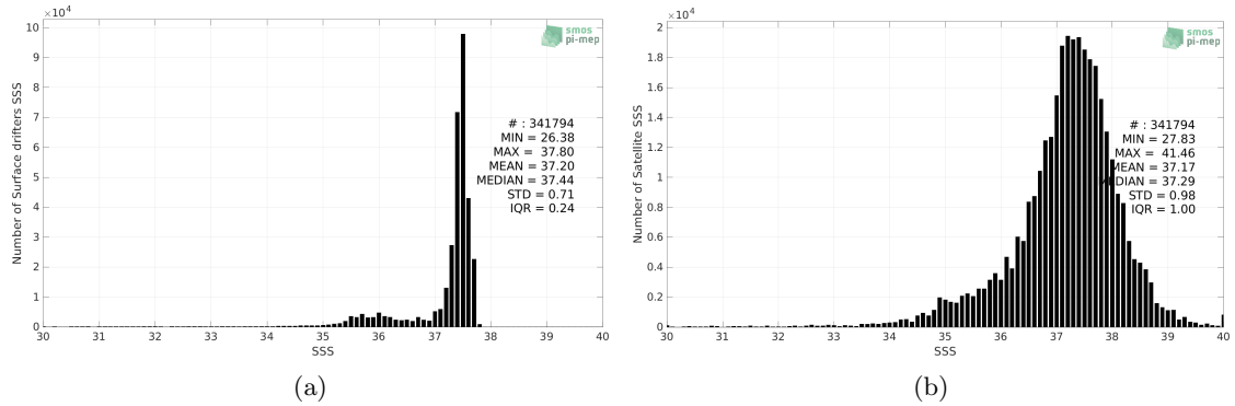
Figure 2: Histograms of SSS from Surface drifters (a) and SMOS SSS L2Q v330 - 0.25 Deg (CATDS-CPDC) (b) considering all match-up pairs per bins of 0.1 over the Amazon and Orinoco river plumes Pi-MEP region and for the full satellite product period.
