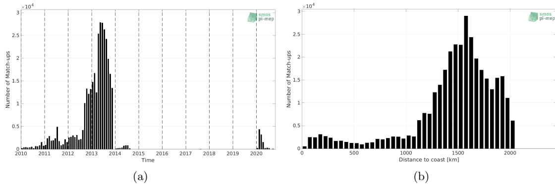
Figure 1: Number of match-ups between Surface drifters and SMOS SSS L2Q v330 - 0.25 Deg (CATDS-CPDC) SSS as a function of time (a) and as function of the distance to coast (b) over the Amazon and Orinoco river plumes Pi-MEP region and for the full satellite product period.
