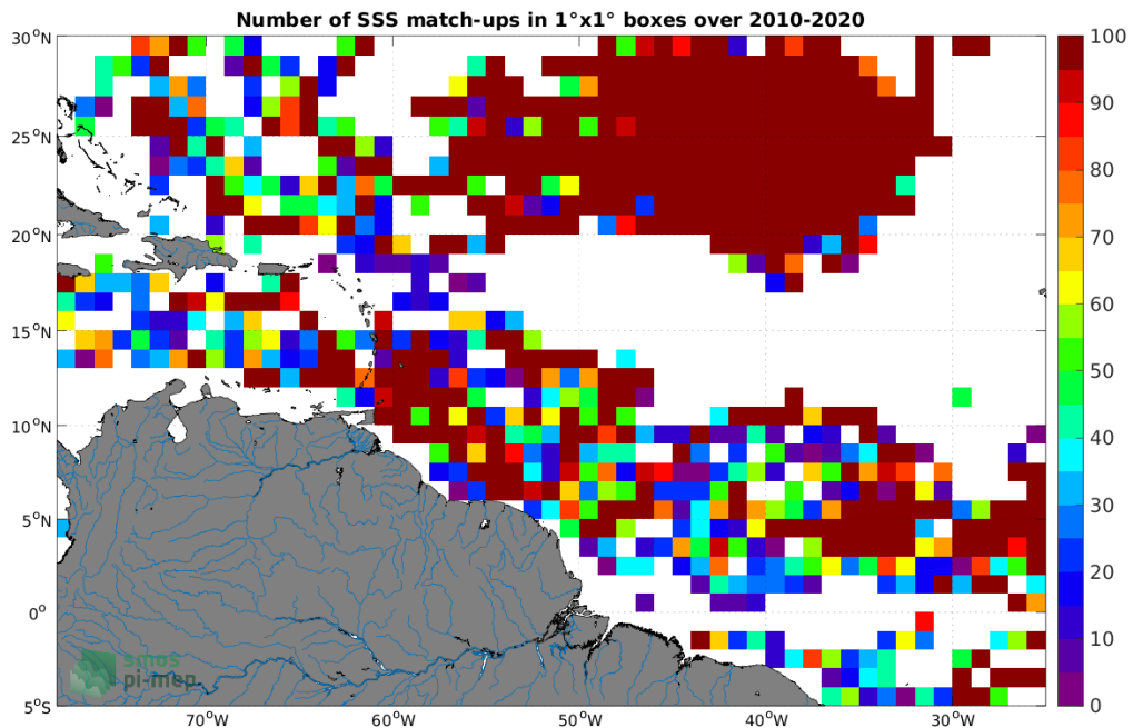
Figure 3: Number of SSS match-ups between Surface drifters SSS and the SMOS SSS L2Q v330 - 0.25 Deg (CATDS-CPDC) SSS product for the Amazon and Orinoco river plumes Pi-MEP region over 1^\circ \times 1^\circ boxes and for the full satellite product period.
