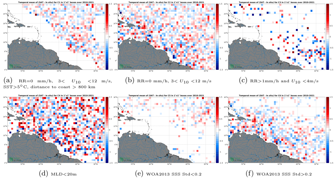
Figure 12: Temporal mean gridded over spatial boxes of size 1^\circ \times 1^\circ of \Delta SSS (SMOS SSS L2Q v330 - 0.25 Deg (CATDS-CPDC) - Argo) for 6 different subdatasets corresponding to: RR=0 mm/h, 3 < U_{10} < 12 m/s, SST >5^\circ C, distance to coast > 800 km (a), RR=0 mm/h, 3 < U_{10} < 12 m/s (b), RR >1 mm/h and U_{10} < 4 m/s (c),MLD <20 m (d),WOA2013 SSS Std <0.2 (e),WOA2013 SSS Std >0.2 (f).
