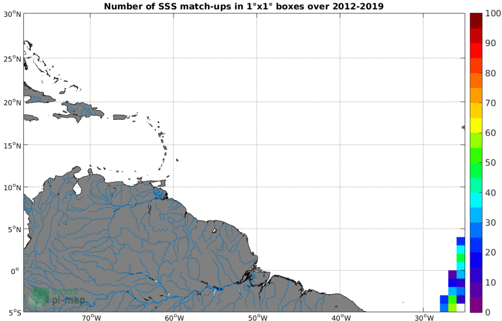
Figure 4: Number of SSS match-ups between TSG (Polarstern) SSS and the SMOS SSS L2Q v321 - 0.25 Deg (CATDS-CPDC) SSS product for the Amazon and Orinoco river plumes Pi-MEP region over 1^\circ \times 1^\circ boxes and for the full satellite product period.
