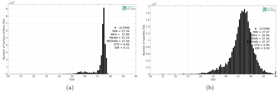
Figure 2: Histograms of SSS from Surface drifters (a) and SMOS SSS L2Q v321 - 0.25 Deg (CATDS-CPDC) (b) considering all match-up pairs per bins of 0.1 over the Amazon and Orinoco river plumes Pi-MEP region and for the full satellite product period.
