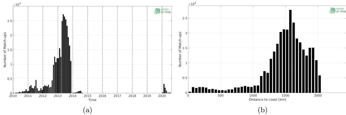
Figure 1: Number of match-ups between Surface drifters and SMOS SSS L2Q v321 - 0.25 Deg (CATDS-CPDC) SSS as a function of time (a) and as function of the distance to coast (b) over the Amazon and Orinoco river plumes Pi-MEP region and for the full satellite product period.
