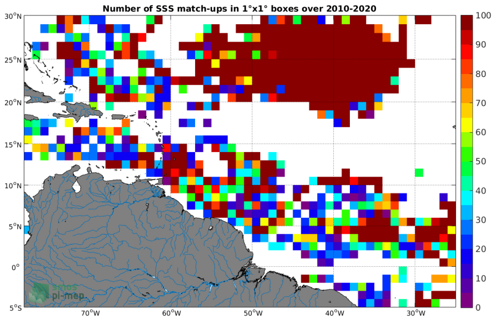
Figure 3: Number of SSS match-ups between Surface drifters SSS and the SMOS SSS L2Q v321 - 0.25 Deg (CATDS-CPDC) SSS product for the Amazon and Orinoco river plumes Pi-MEP region over 1^\circ \times 1^\circ boxes and for the full satellite product period.
