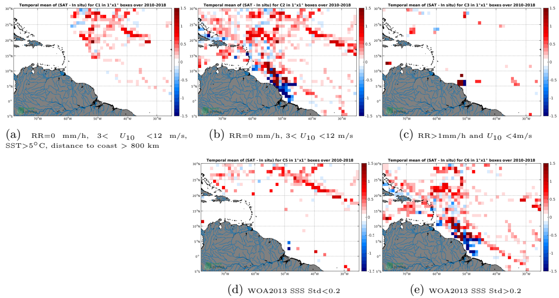
Figure 12: Temporal mean gridded over spatial boxes of size 1^\circ \times 1^\circ of \Delta SSS (SMOS-L3-CATDS-CPDC-V317-MONTHLY-25KM - TSG-SAMOS) for 5 different subdatasets corresponding to:RR=0 mm/h, 3 < U_{10} < 12 m/s, SST >5^\circ C, distance to coast > 800 km (a), RR=0 mm/h, 3 < U_{10} < 12 m/s (b), RR >1 mm/h and U_{10} < 4 m/s (c), WOA2013 SSS Std <0.2 (d), WOA2013 SSS Std >0.2 (e).
