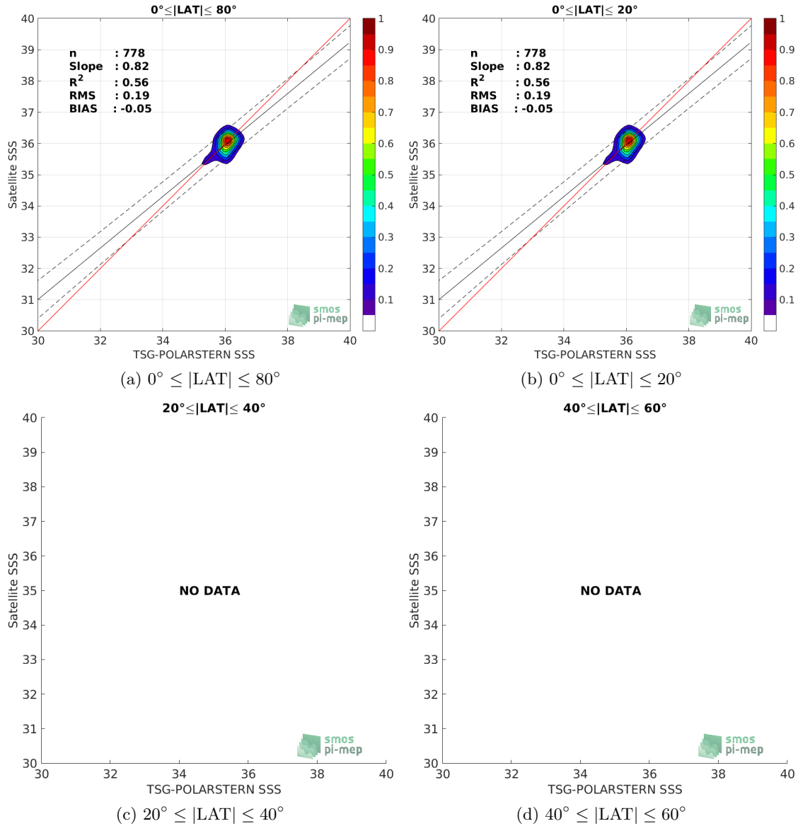
Figure 9: Contour maps of the concentration of SMOS-L3-CATDS-CPDC-V317-MONTHLY-25KM SSS (y-axis) versus TSG-POLARSTERN SSS (x-axis) at match-up pairs for different latitude bands. For each plot, the red line shows x=y . The black thin and dashed lines indicate a linear fit through the data cloud and the \pm 95\% confidence levels, respectively. The number match-up pairs n , the slope and R^2 coefficient of the linear fit, the root mean square (RMS) and the mean bias between satellite and in situ data are indicated for each latitude band in each plots.
