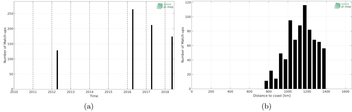
Figure 1: Number of match-ups between TSG-POLARSTERN and SMOS-L3-CATDS-CPDC-V317-MONTHLY-25KM SSS as a function of time (a) and as function of the distance to coast (b) over the Amazon and Orinoco river plumes Pi-MEP region and for the full satellite product period.
