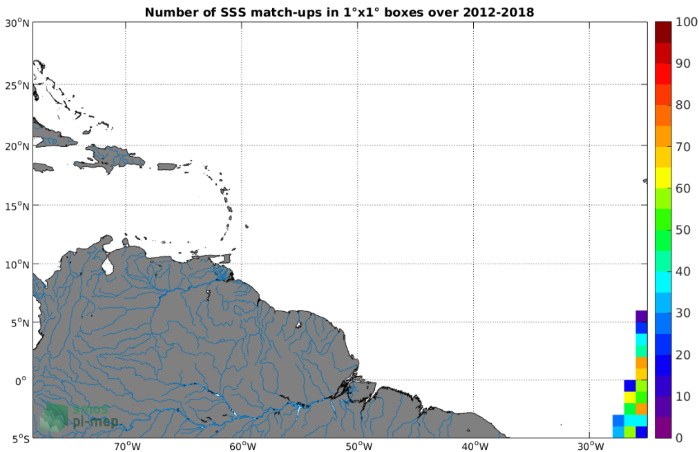
Figure 4: Number of SSS match-ups between TSG-POLARSTERN SSS and the SMOS-L3-CATDS-CPDC-V317-MONTHLY-25KM SSS product for the Amazon and Orinoco river plumes Pi-MEP region over 1^\circ \times 1^\circ boxes and for the full satellite product period.
