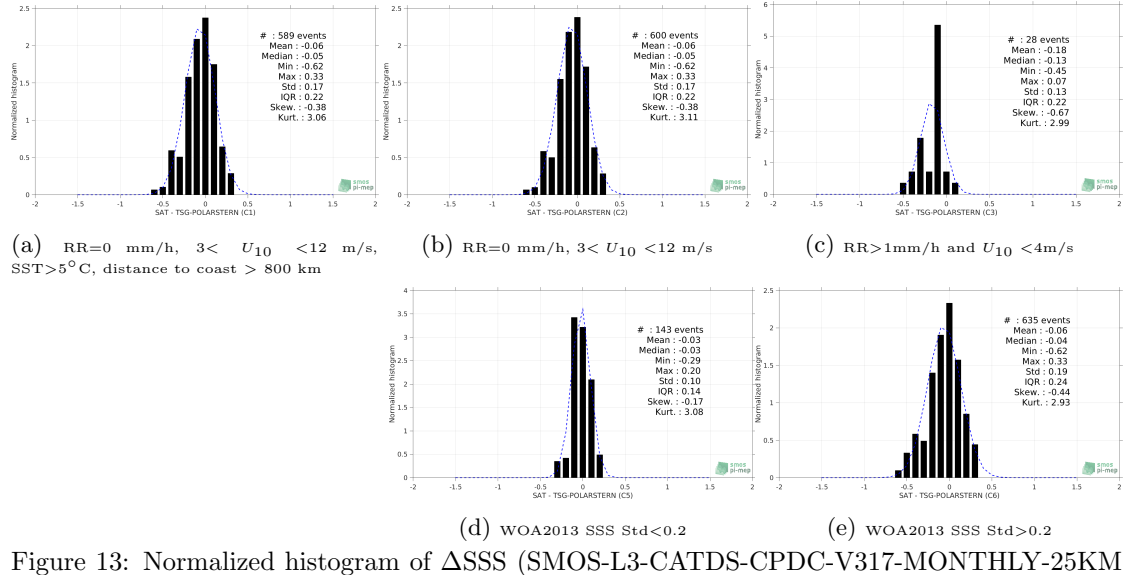
Figure 13: Normalized histogram of \Delta SSS (SMOS-L3-CATDS-CPDC-V317-MONTHLY-25KM - TSG-POLARSTERN) for 5 different subdatasets corresponding to: RR=0 mm/h, 3 < U_{10} < 12 m/s, SST > 5^\circ C , distance to coast > 800 km (a), RR=0 mm/h, 3 < U_{10} < 12 m/s (b), RR > 1 mm/h and U_{10} < 4 m/s (c), WOA2013 SSS Std < 0.2 (d), WOA2013 SSS Std > 0.2 (e).
