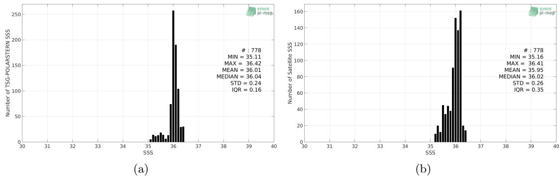
Figure 2: Histograms of SSS from TSG-POLARSTERN (a) and SMOS-L3-CATDS-CPDC-V317-MONTHLY-25KM (b) considering all match-up pairs per bins of 0.1 over the Amazon and Orinoco river plumes Pi-MEP region and for the full satellite product period.
