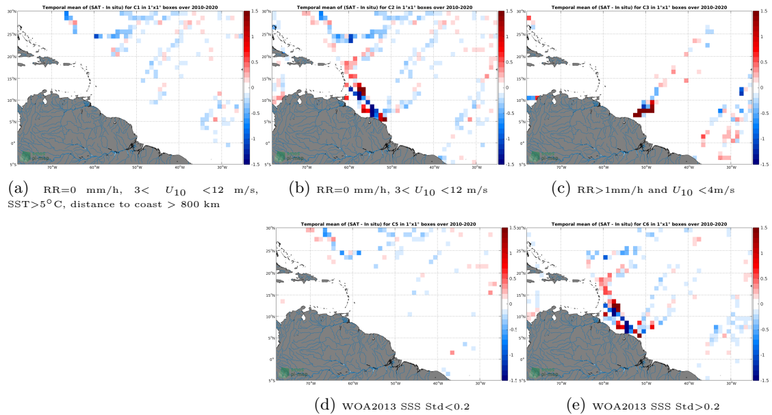
Figure 12: Temporal mean gridded over spatial boxes of size 1^{\circ}\times 1^{\circ} of \Delta\text{SSS} (SMOS SSS L3 v317 - Monthly - 25 km (CATDS-CPDC) - TSG (LEGOS-DM)) for 5 different subdatasets corresponding to:RR=0 mm/h, 3 < U_{10} < 12 m/s, SST >5^{\circ}\text{C} , distance to coast > 800 km (a), RR=0 mm/h, 3 < U_{10} < 12 m/s (b), RR >1 mm/h and U_{10} < 4 m/s (c), WOA2013 SSS Std <0.2 (d), WOA2013 SSS Std >0.2 (e).
