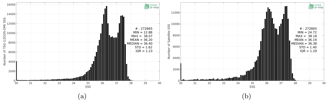
Figure 2: Histograms of SSS from TSG (LEGOS-DM) (a) and SMOS SSS L3 v317 - Monthly - 25 km (CATDS-CPDC) (b) considering all match-up pairs per bins of 0.1 over the Amazon and Orinoco river plumes Pi-MEP region and for the full satellite product period.
