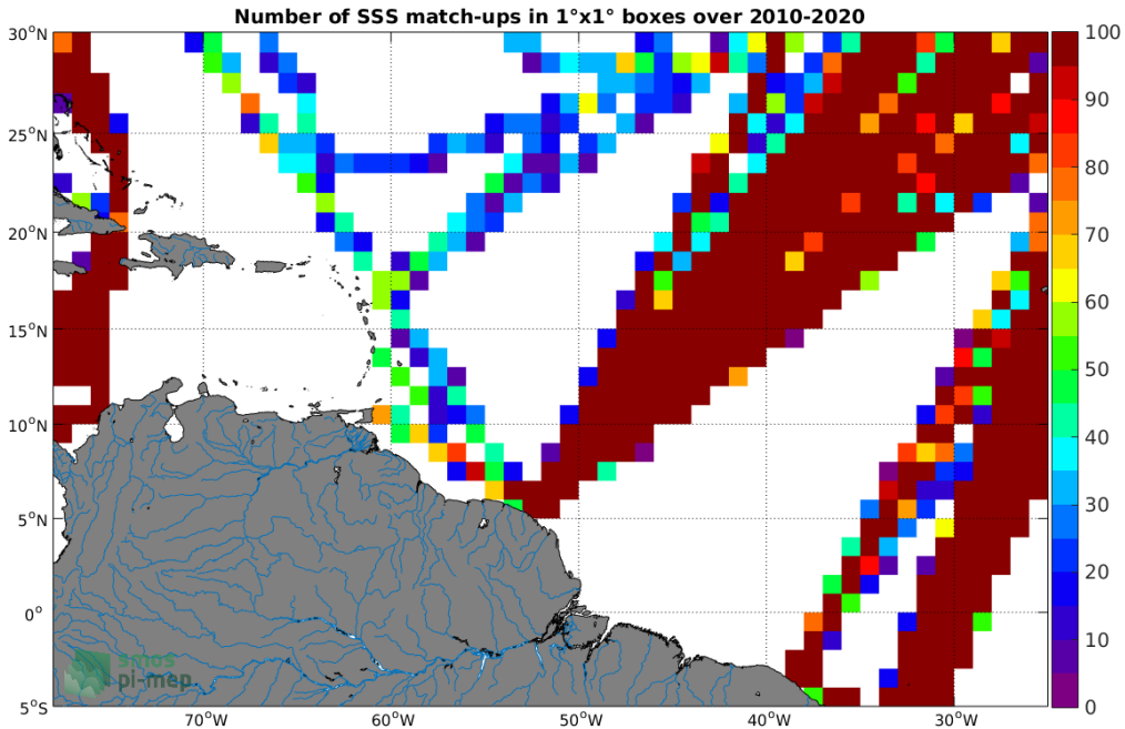
Figure 4: Number of SSS match-ups between TSG (LEGOS-DM) SSS and the SMOS SSS L3 v317 - Monthly - 25 km (CATDS-CPDC) SSS product for the Amazon and Orinoco river plumes Pi-MEP region over 1^\circ \times 1^\circ boxes and for the full satellite product period.
