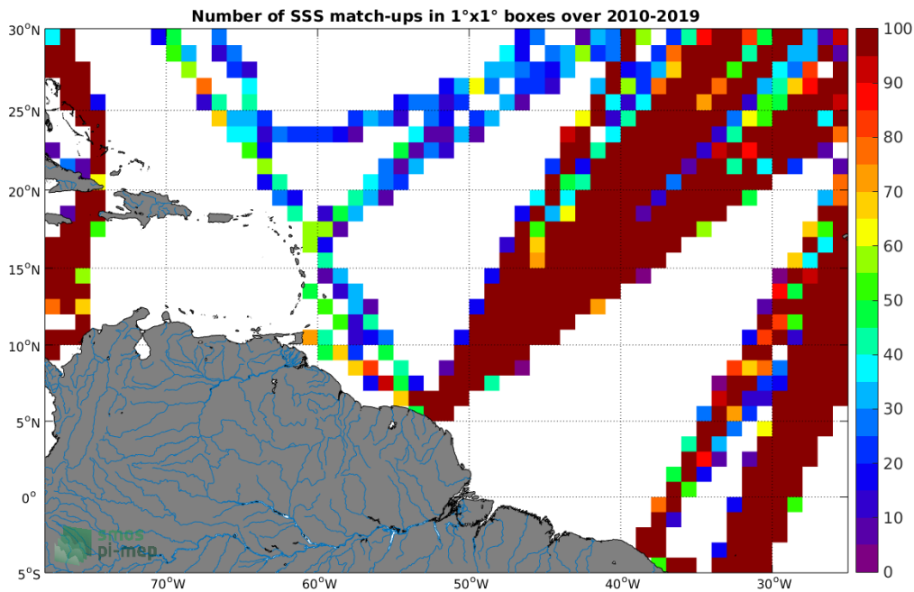
Figure 4: Number of SSS match-ups between TSG-LEGOS-DM SSS and the SMOS L3 v317 - Monthly - 25 km (CATDS-CPDC) SSS product for the Amazon and Orinoco river plumes Pi-MEP region over 1°x1° boxes and for the full satellite product period.
