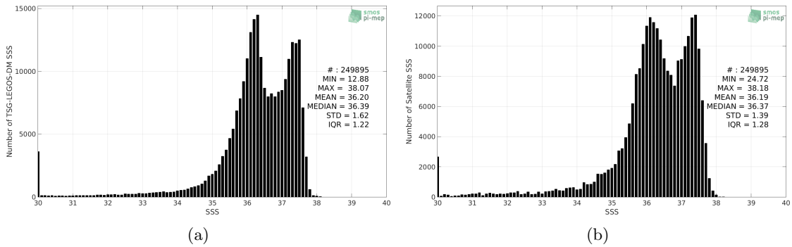
Figure 2: Histograms of SSS from TSG-LEGOS-DM (a) and SMOS L3 v317 - Monthly - 25 km (CATDS-CPDC) (b) considering all match-up pairs per bins of 0.1 over the Amazon and Orinoco river plumes Pi-MEP region and for the full satellite product period.
