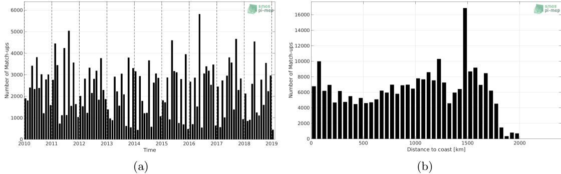
Figure 1: Number of match-ups between TSG-LEGOS-DM and SMOS L3 v317 - Monthly - 25 km (CATDS-CPDC) SSS as a function of time (a) and as function of the distance to coast (b) over the Amazon and Orinoco river plumes Pi-MEP region and for the full satellite product period.
