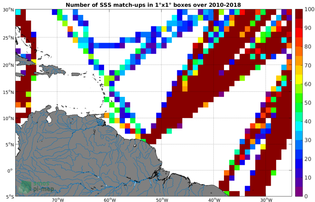
Figure 4: Number of SSS match-ups between TSG-LEGOS-DM SSS and the SMOS-L3-CATDS-CPDC-V317-MONTHLY-25KM SSS product for the Amazon and Orinoco river plumes Pi-MEP region over 1°x1° boxes and for the full satellite product period.
