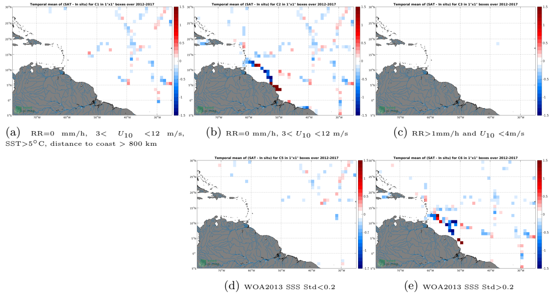
Figure 12: Temporal mean gridded over spatial boxes of size 1^{\circ}\times 1^{\circ} of \Delta SSS (SMOS SSS L3 v317 - Monthly - 25 km (CATDS-CPDC) - TSG (GOSUD-Sailing-ship)) for 5 different subdatasets corresponding to:RR=0 mm/h, 3 < U_{10} < 12 m/s, SST >5^{\circ}\text{C} , distance to coast > 800 km (a), RR=0 mm/h, 3 < U_{10} < 12 m/s (b), RR >1 mm/h and U_{10} < 4 m/s (c), WOA2013 SSS Std <0.2 (d), WOA2013 SSS Std >0.2 (e).
