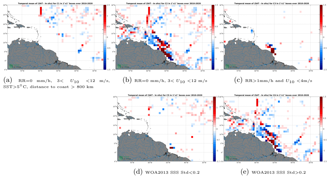
Figure 12: Temporal mean gridded over spatial boxes of size 1^\circ \times 1^\circ of \Delta SSS (SMOS SSS L3 v317 - Monthly - 25 km (CATDS-CPDC) - TSG (GOSUD-Research-vessel)) for 5 different subdatasets corresponding to:RR=0 mm/h, 3 < U_{10} < 12 m/s, SST >5^\circ\text{C} , distance to coast > 800 km (a), RR=0 mm/h, 3 < U_{10} < 12 m/s (b), RR >1 mm/h and U_{10} < 4 m/s (c), WOA2013 SSS Std <0.2 (d), WOA2013 SSS Std >0.2 (e).
