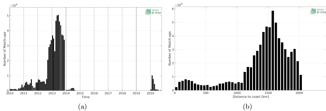
Figure 1: Number of match-ups between Surface drifters and SMOS SSS L3 v317 - Monthly - 25 km (CATDS-CPDC) SSS as a function of time (a) and as function of the distance to coast (b) over the Amazon and Orinoco river plumes Pi-MEP region and for the full satellite product period.
