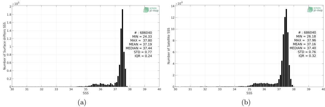
Figure 2: Histograms of SSS from Surface drifters (a) and SMOS L3 v317 - Monthly - 25 km (CATDS-CPDC) (b) considering all match-up pairs per bins of 0.1 over the Amazon and Orinoco river plumes Pi-MEP region and for the full satellite product period.
