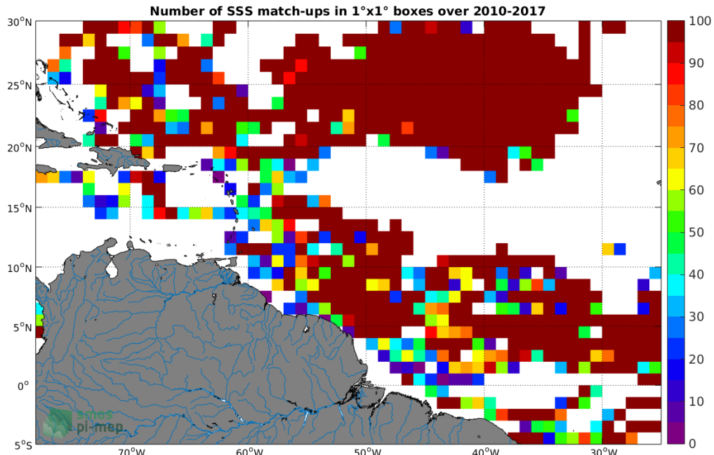
Figure 3: Number of SSS match-ups between Surface drifters SSS and the SMOS L3 v317 - Monthly - 25 km (CATDS-CPDC) SSS product for the Amazon and Orinoco river plumes Pi-MEP region over 1°x1° boxes and for the full satellite product period.
