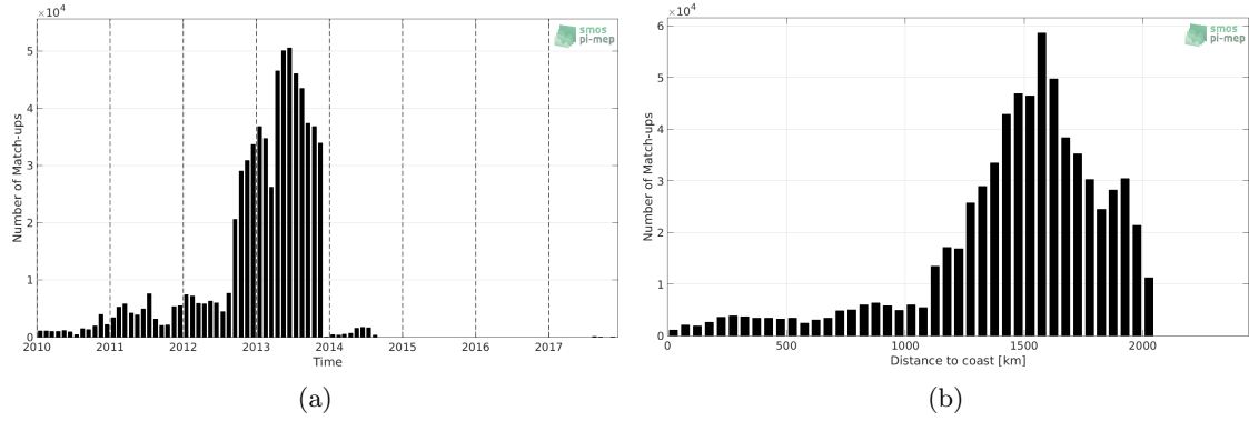
Figure 1: Number of match-ups between Surface drifters and SMOS L3 v317 - Monthly - 25 km (CATDS-CPDC) SSS as a function of time (a) and as function of the distance to coast (b) over the Amazon and Orinoco river plumes Pi-MEP region and for the full satellite product period.
