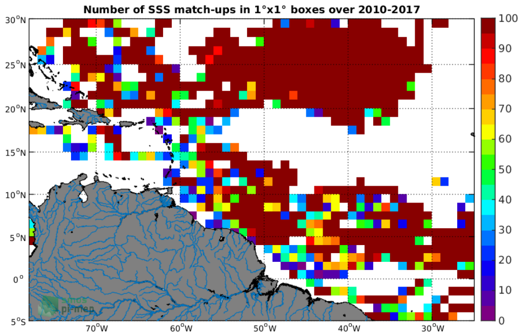
Figure 3: Number of SSS match-ups between Surface drifters SSS and the SMOS-L3-CATDS-CPDC-V317-MONTHLY-25KM SSS product for the Amazon and Orinoco river plumes Pi-MEP region over 1^\circ \times 1^\circ boxes and for the full satellite product period.
