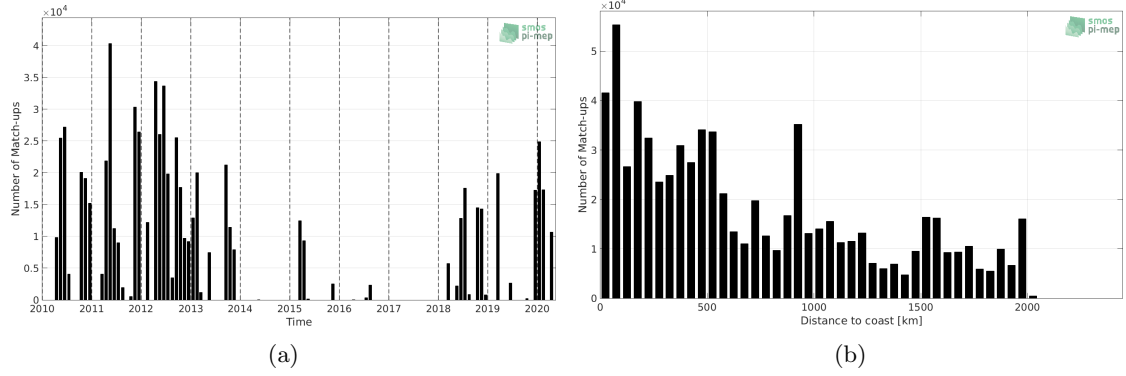
Figure 1: Number of match-ups between TSG (SAMOS) and SMOS SSS L3 v317 - 10 Days - 25 km (CATDS-CPDC) SSS as a function of time (a) and as function of the distance to coast (b) over the Amazon and Orinoco river plumes Pi-MEP region and for the full satellite product period.
