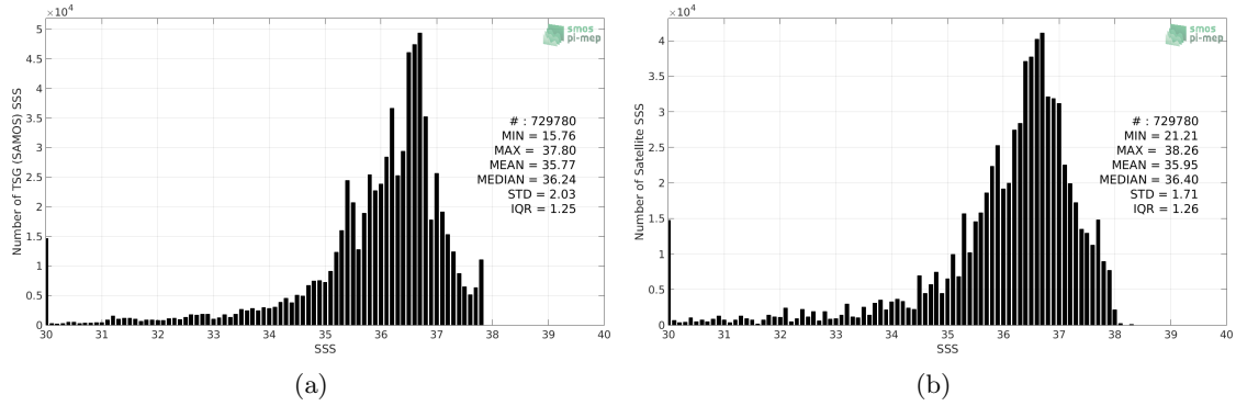
Figure 2: Histograms of SSS from TSG (SAMOS) (a) and SMOS SSS L3 v317 - 10 Days - 25 km (CATDS-CPDC) (b) considering all match-up pairs per bins of 0.1 over the Amazon and Orinoco river plumes Pi-MEP region and for the full satellite product period.
