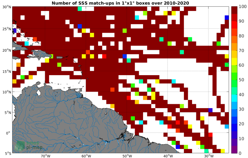
Figure 4: Number of SSS match-ups between TSG (SAMOS) SSS and the SMOS SSS L3 v317 - 10 Days - 25 km (CATDS-CPDC) SSS product for the Amazon and Orinoco river plumes Pi-MEP region over 1^\circ \times 1^\circ boxes and for the full satellite product period.
