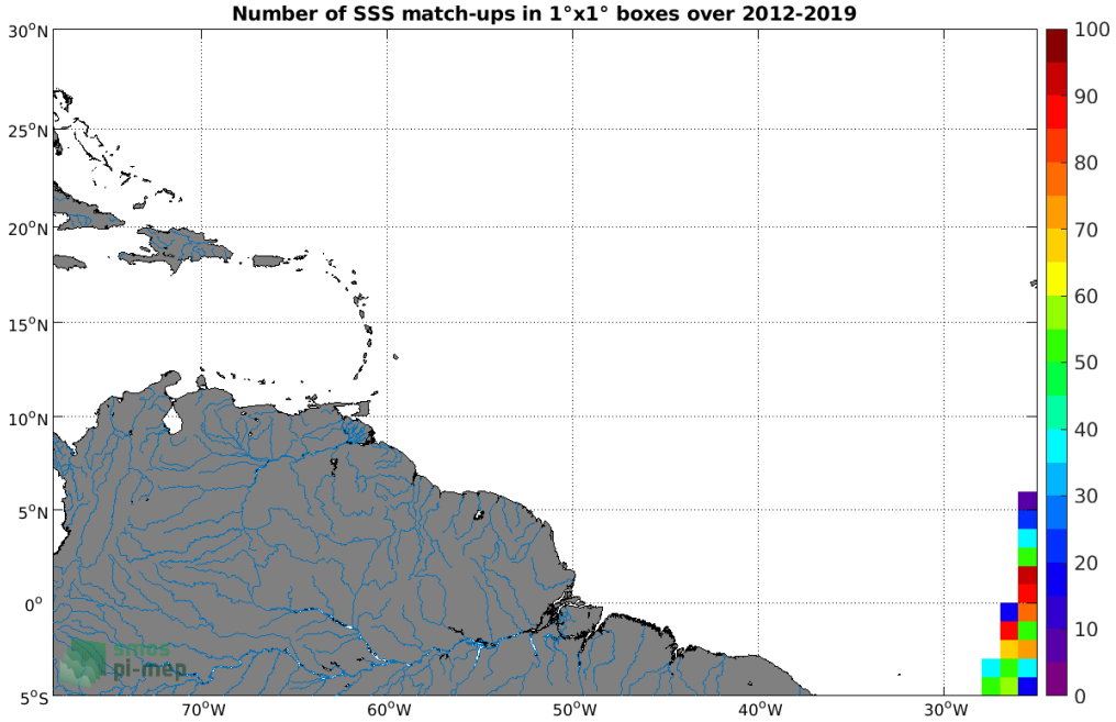
Figure 4: Number of SSS match-ups between TSG (Polarstern) SSS and the SMOS SSS L3 v317 - 10 Days - 25 km (CATDS-CPDC) SSS product for the Amazon and Orinoco river plumes Pi-MEP region over 1^\circ \times 1^\circ boxes and for the full satellite product period.
