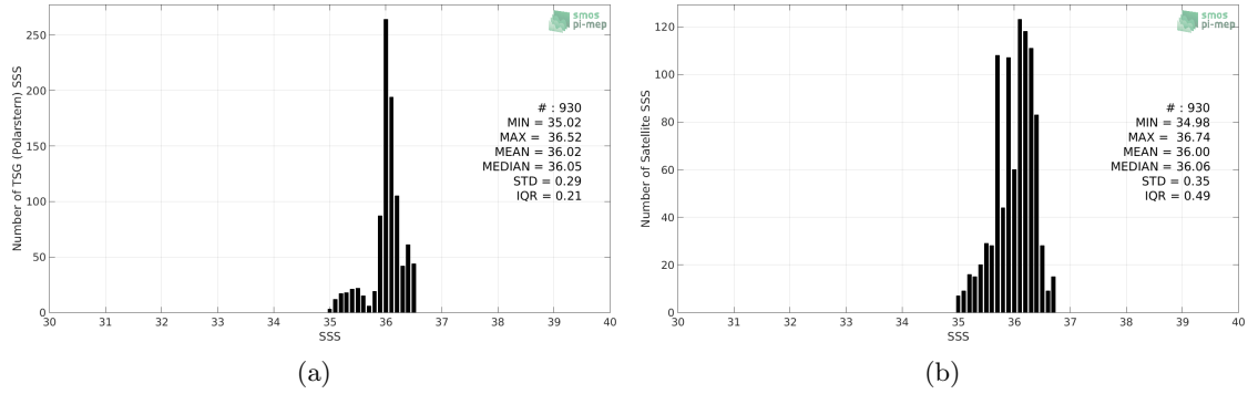
Figure 2: Histograms of SSS from TSG (Polarstern) (a) and SMOS SSS L3 v317 - 10 Days - 25 km (CATDS-CPDC) (b) considering all match-up pairs per bins of 0.1 over the Amazon and Orinoco river plumes Pi-MEP region and for the full satellite product period.
