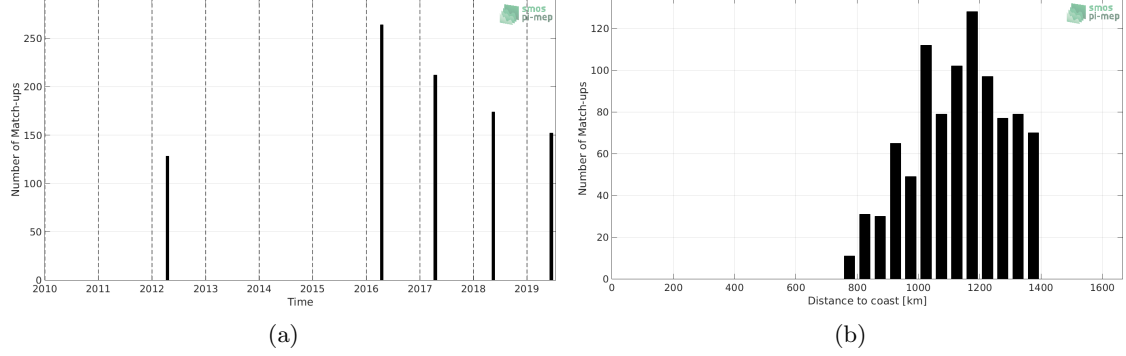
Figure 1: Number of match-ups between TSG (Polarstern) and SMOS SSS L3 v317 - 10 Days - 25 km (CATDS-CPDC) SSS as a function of time (a) and as function of the distance to coast (b) over the Amazon and Orinoco river plumes Pi-MEP region and for the full satellite product period.
