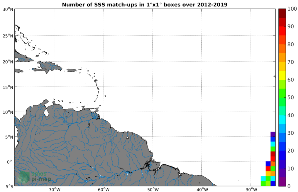
Figure 4: Number of SSS match-ups between TSG (Polarstern) SSS and the SMOS SSS L3 v317 - 10 Days - 25 km (CATDS-CPDC) SSS product for the Amazon and Orinoco river plumes Pi-MEP region over 1°x1° boxes and for the full satellite product period.
