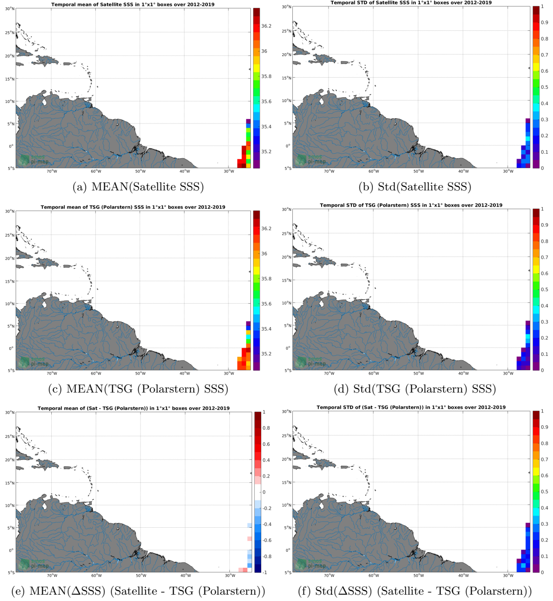
Figure 6: Temporal mean (left) and Std (right) of SSS from SMOS SSS L3 v317 - 10 Days - 25 km (CATDS-CPDC) (top), TSG (Polarstern) (middle), and of \Delta SSS (Satellite - TSG (Polarstern)). Only match-up pairs are used to generate these maps.
