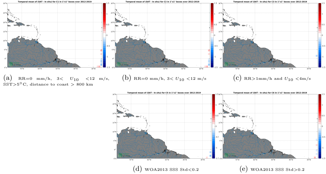
Figure 12: Temporal mean gridded over spatial boxes of size 1^{\circ}\times 1^{\circ} of \Delta\text{SSS} (SMOS L3 v317 - 10 Days - 25 km (CATDS-CPDC) - TSG-POLARSTERN) for 5 different subdatasets corresponding to: \text{RR}=0 mm/h, 3 < U_{10} < 12 m/s, \text{SST} > 5^{\circ}\text{C} , distance to coast > 800 km (a), \text{RR}=0 mm/h, 3 < U_{10} < 12 m/s (b), \text{RR} > 1 mm/h and U_{10} < 4 m/s (c), WOA2013 SSS Std < 0.2 (d), WOA2013 SSS Std > 0.2 (e).
