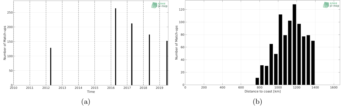
Figure 1: Number of match-ups between TSG-POLARSTERN and SMOS L3 v317 - 10 Days - 25 km (CATDS-CPDC) SSS as a function of time (a) and as function of the distance to coast (b) over the Amazon and Orinoco river plumes Pi-MEP region and for the full satellite product period.
