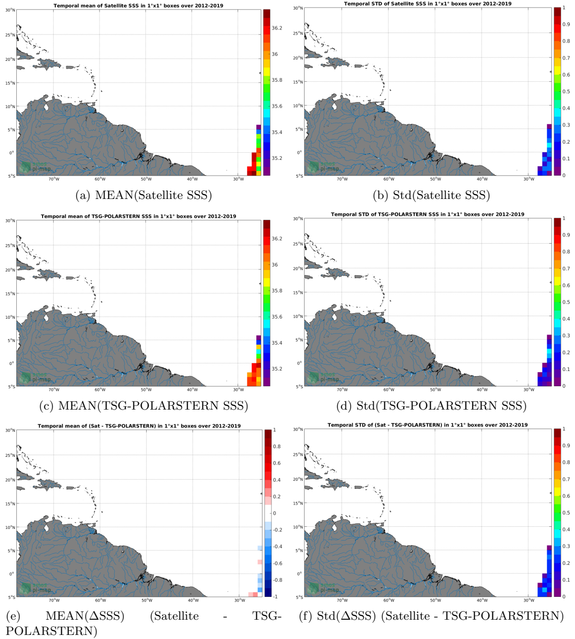
Figure 6: Temporal mean (left) and Std (right) of SSS from SMOS L3 v317 - 10 Days - 25 km (CATDS-CPDC) (top), TSG-POLARSTERN (middle), and of \Delta SSS (Satellite - TSG-POLARSTERN). Only match-up pairs are used to generate these maps.
