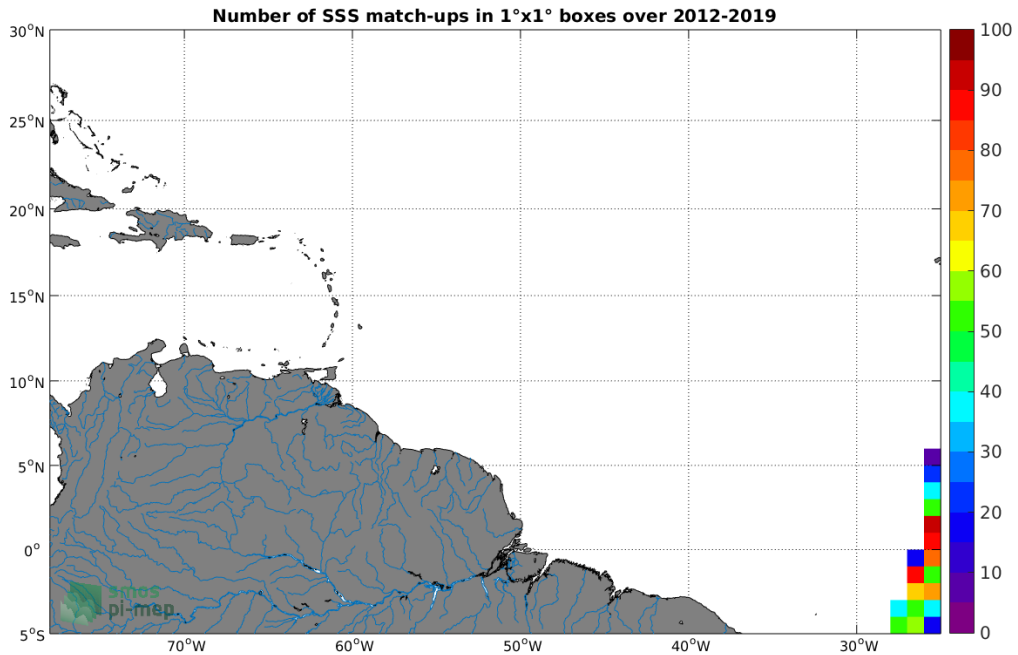
Figure 4: Number of SSS match-ups between TSG-POLARSTERN SSS and the SMOS L3 v317 - 10 Days - 25 km (CATDS-CPDC) SSS product for the Amazon and Orinoco river plumes Pi-MEP region over 1^\circ \times 1^\circ boxes and for the full satellite product period.
