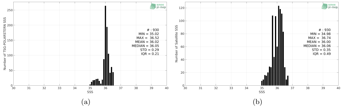
Figure 2: Histograms of SSS from TSG-POLARSTERN (a) and SMOS L3 v317 - 10 Days - 25 km (CATDS-CPDC) (b) considering all match-up pairs per bins of 0.1 over the Amazon and Orinoco river plumes Pi-MEP region and for the full satellite product period.
