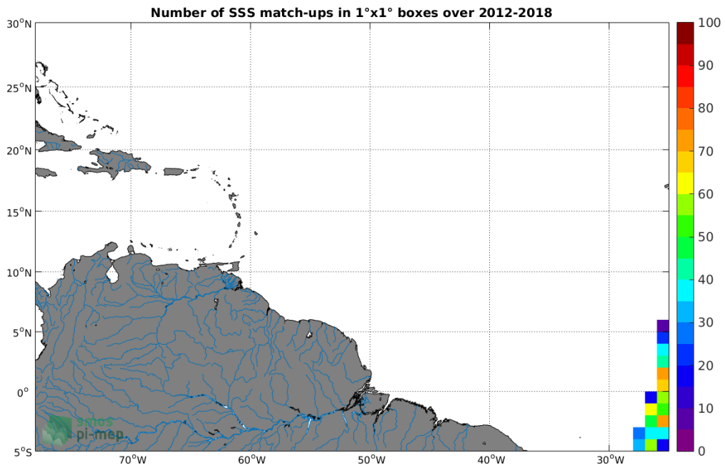
Figure 4: Number of SSS match-ups between TSG-POLARSTERN SSS and the SMOS-L3-CATDS-CPDC-V317-10DAYS-25KM SSS product for the Amazon and Orinoco river plumes Pi-MEP region over 1^\circ \times 1^\circ boxes and for the full satellite product period.
