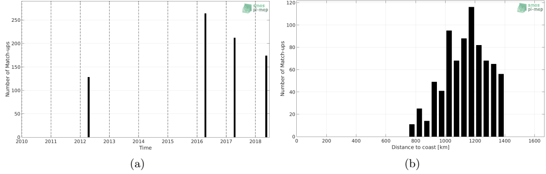
Figure 1: Number of match-ups between TSG-POLARSTERN and SMOS-L3-CATDS-CPDC-V317-10DAYS-25KM SSS as a function of time (a) and as function of the distance to coast (b) over the Amazon and Orinoco river plumes Pi-MEP region and for the full satellite product period.
