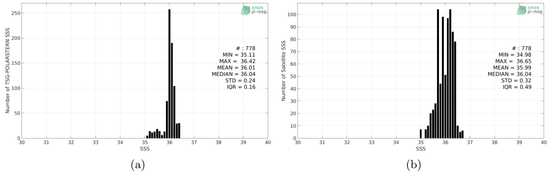
Figure 2: Histograms of SSS from TSG-POLARSTERN (a) and SMOS-L3-CATDS-CPDC-V317-10DAYS-25KM (b) considering all match-up pairs per bins of 0.1 over the Amazon and Orinoco river plumes Pi-MEP region and for the full satellite product period.
