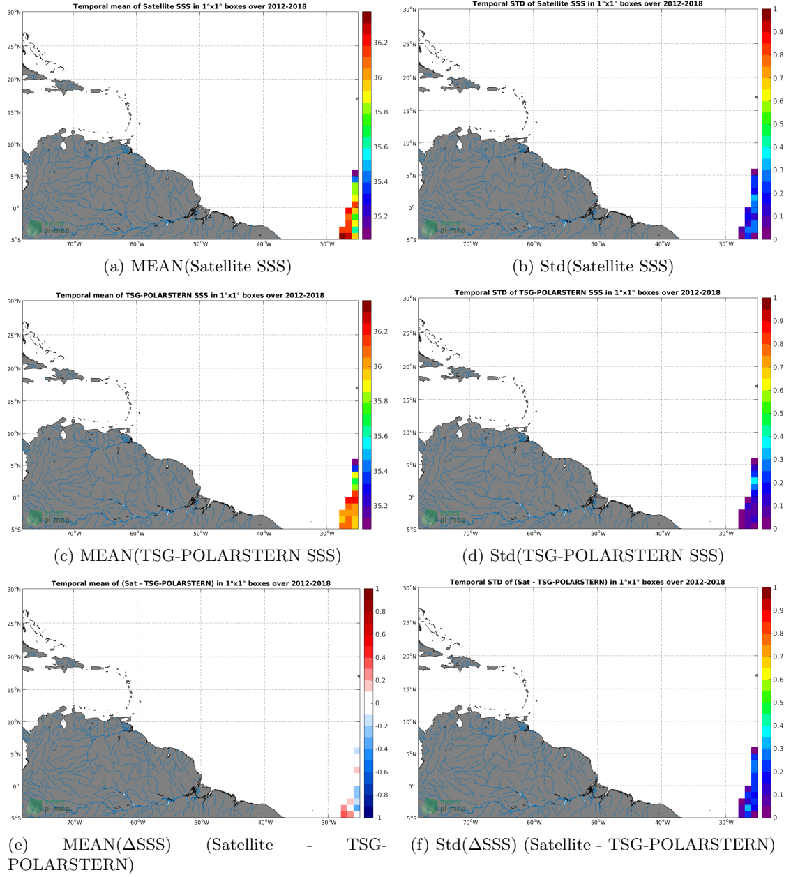
Figure 6: Temporal mean (left) and Std (right) of SSS from SMOS-L3-CATDS-CPDC-V317-10DAYS-25KM (top), TSG-POLARSTERN (middle), and of \Delta SSS (Satellite - TSG-POLARSTERN). Only match-up pairs are used to generate these maps.
