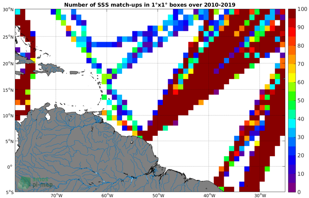
Figure 4: Number of SSS match-ups between TSG (LEGOS-DM) SSS and the SMOS SSS L3 v317 - 10 Days - 25 km (CATDS-CPDC) SSS product for the Amazon and Orinoco river plumes Pi-MEP region over 1°x1° boxes and for the full satellite product period.
