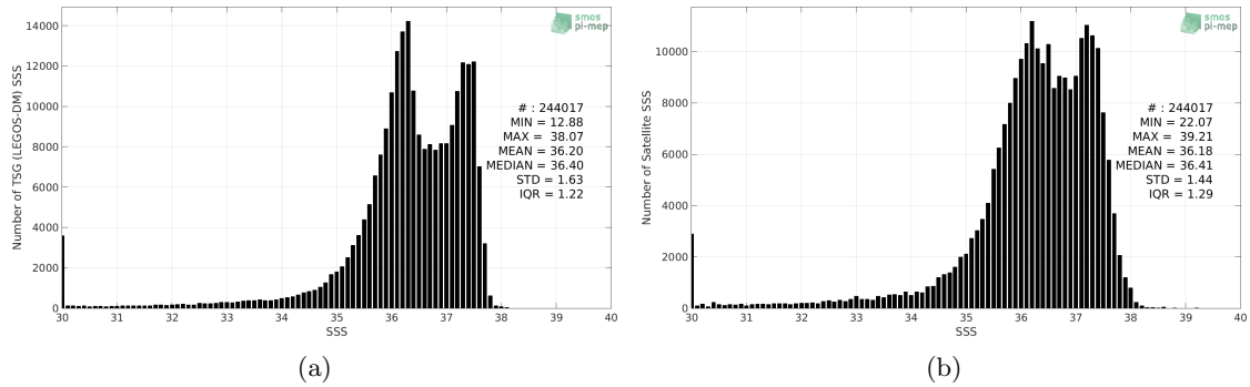
Figure 2: Histograms of SSS from TSG (LEGOS-DM) (a) and SMOS SSS L3 v317 - 10 Days - 25 km (CATDS-CPDC) (b) considering all match-up pairs per bins of 0.1 over the Amazon and Orinoco river plumes Pi-MEP region and for the full satellite product period.
