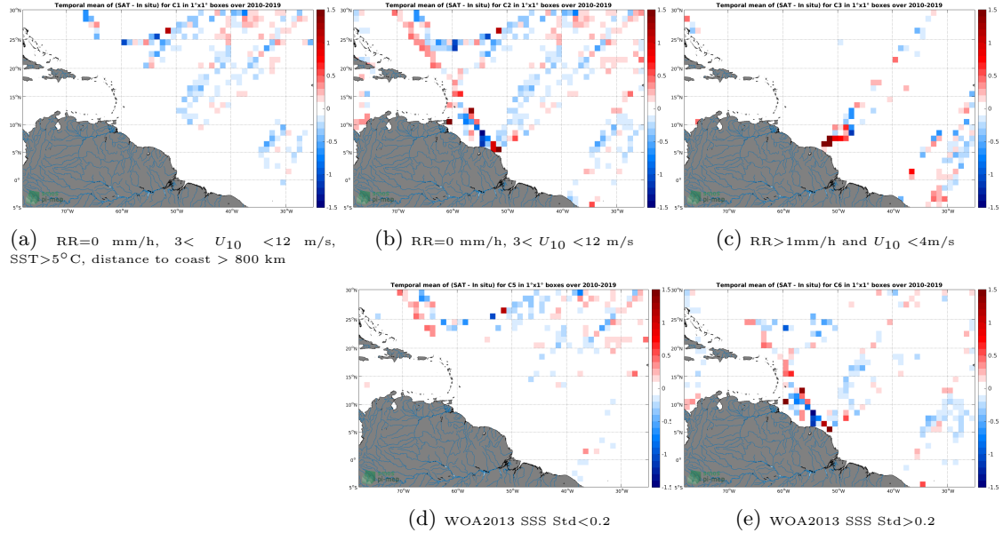
Figure 12: Temporal mean gridded over spatial boxes of size 1^{\circ}\times 1^{\circ} of \Delta\text{SSS} (SMOS SSS L3 v317 - 10 Days - 25 km (CATDS-CPDC) - TSG (LEGOS-DM)) for 5 different subdatasets corresponding to:RR=0 mm/h, 3 < U_{10} < 12 m/s, SST >5^{\circ}\text{C} , distance to coast > 800 km (a), RR=0 mm/h, 3 < U_{10} < 12 m/s (b), RR >1 mm/h and U_{10} < 4 m/s (c), WOA2013 SSS Std <0.2 (d), WOA2013 SSS Std >0.2 (e).
