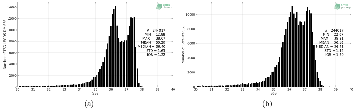
Figure 2: Histograms of SSS from TSG-LEGOS-DM (a) and SMOS L3 v317 - 10 Days - 25 km (CATDS-CPDC) (b) considering all match-up pairs per bins of 0.1 over the Amazon and Orinoco river plumes Pi-MEP region and for the full satellite product period.
