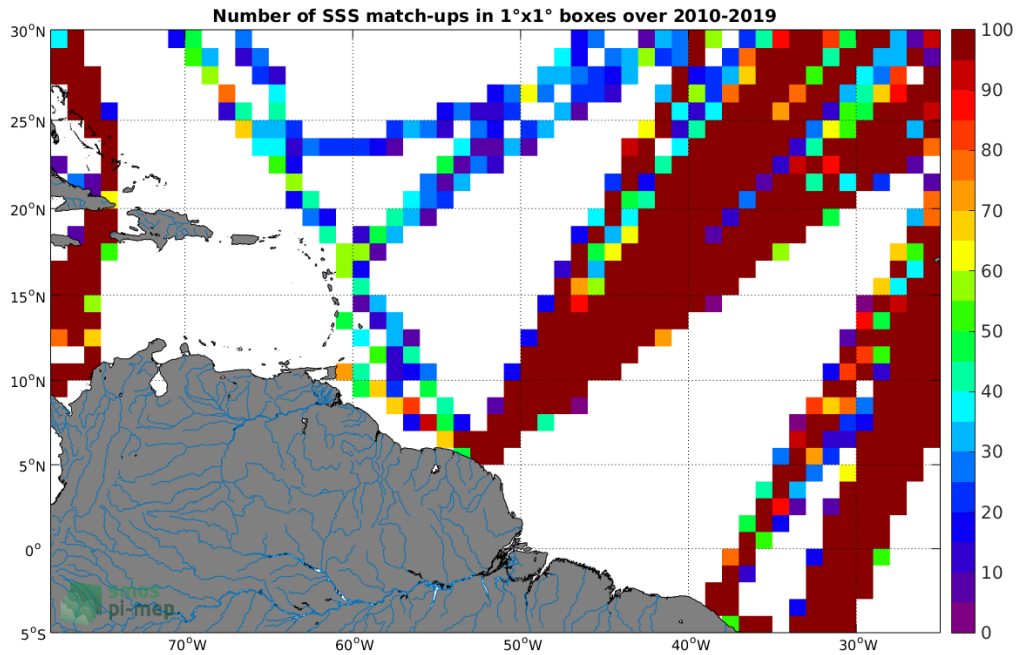
Figure 4: Number of SSS match-ups between TSG-LEGOS-DM SSS and the SMOS L3 v317 - 10 Days - 25 km (CATDS-CPDC) SSS product for the Amazon and Orinoco river plumes Pi-MEP region over 1^\circ \times 1^\circ boxes and for the full satellite product period.
