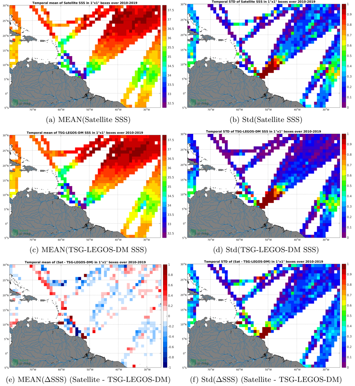
Figure 6: Temporal mean (left) and Std (right) of SSS from SMOS L3 v317 - 10 Days - 25 km (CATDS-CPDC) (top), TSG-LEGOS-DM (middle), and of \Delta SSS (Satellite - TSG-LEGOS-DM). Only match-up pairs are used to generate these maps.
