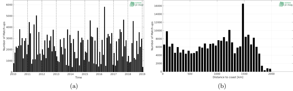
Figure 1: Number of match-ups between TSG-LEGOS-DM and SMOS L3 v317 - 10 Days - 25 km (CATDS-CPDC) SSS as a function of time (a) and as function of the distance to coast (b) over the Amazon and Orinoco river plumes Pi-MEP region and for the full satellite product period.
