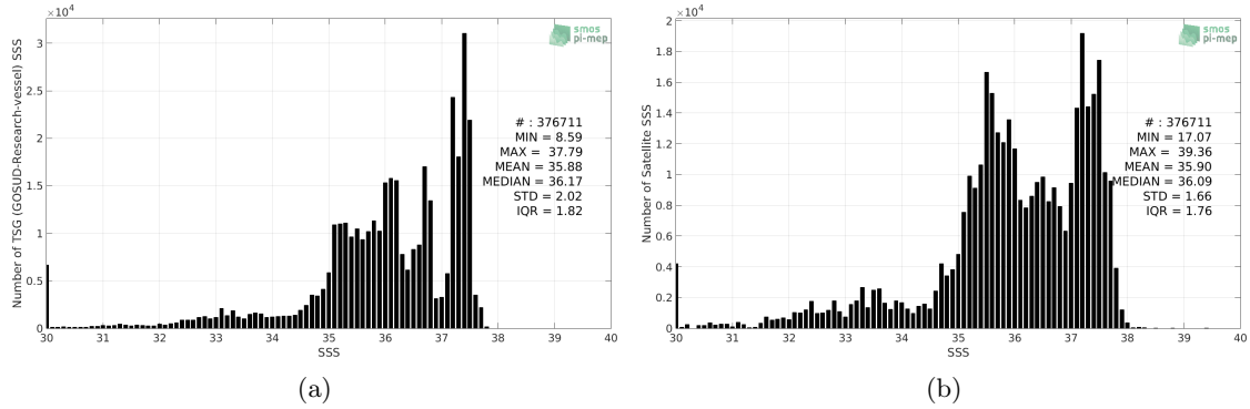
Figure 2: Histograms of SSS from TSG (GOSUD-Research-vessel) (a) and SMOS SSS L3 v317 - 10 Days - 25 km (CATDS-CPDC) (b) considering all match-up pairs per bins of 0.1 over the Amazon and Orinoco river plumes Pi-MEP region and for the full satellite product period.
