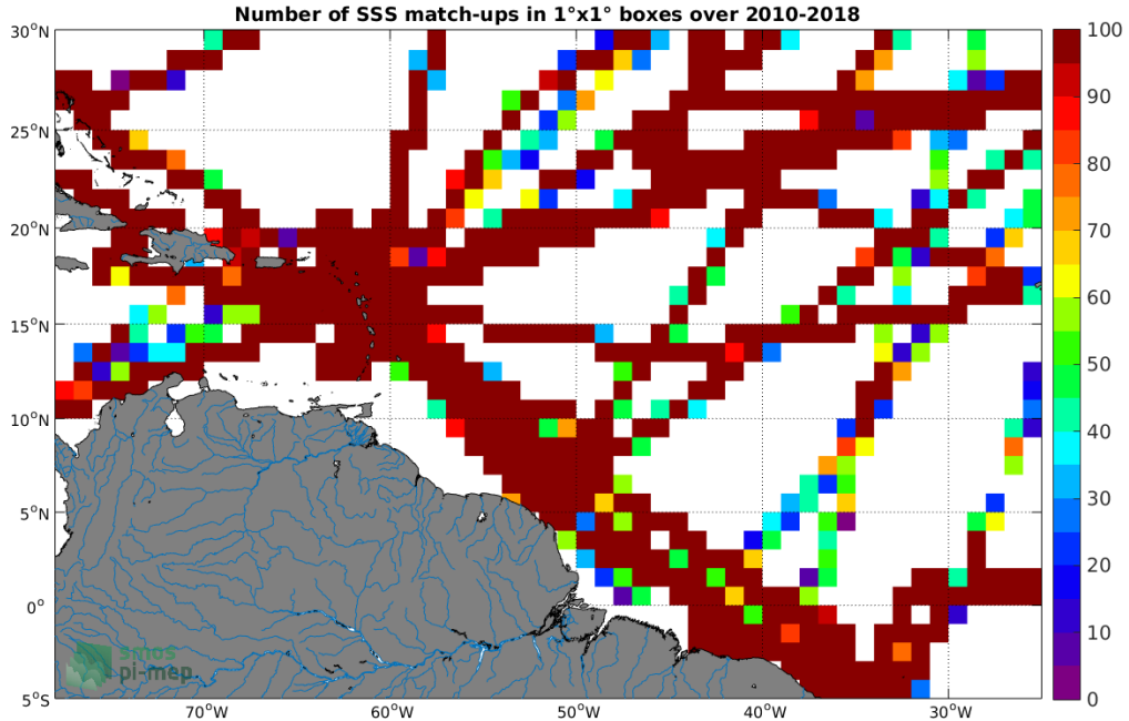
Figure 4: Number of SSS match-ups between TSG (GOSUD-Research-vessel) SSS and the SMOS SSS L3 v317 - 10 Days - 25 km (CATDS-CPDC) SSS product for the Amazon and Orinoco river plumes Pi-MEP region over 1^\circ \times 1^\circ boxes and for the full satellite product period.
