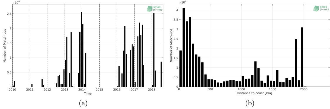
Figure 1: Number of match-ups between TSG-GOSUD-Research-vessel and SMOS L3 v317 - 10 Days - 25 km (CATDS-CPDC) SSS as a function of time (a) and as function of the distance to coast (b) over the Amazon and Orinoco river plumes Pi-MEP region and for the full satellite product period.
