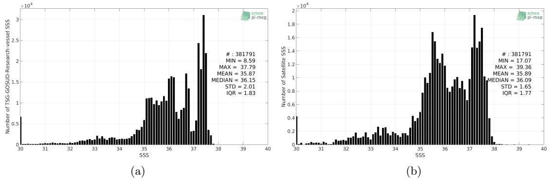
Figure 2: Histograms of SSS from TSG-GOSUD-Research-vessel (a) and SMOS L3 v317 - 10 Days - 25 km (CATDS-CPDC) (b) considering all match-up pairs per bins of 0.1 over the Amazon and Orinoco river plumes Pi-MEP region and for the full satellite product period.
