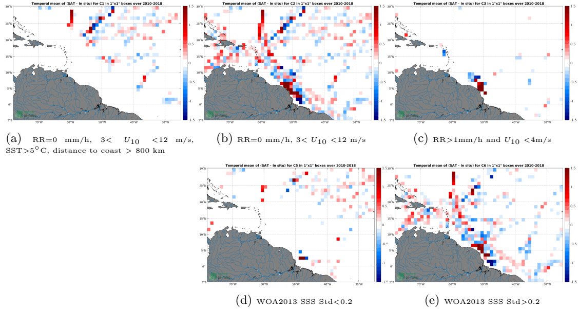
Figure 12: Temporal mean gridded over spatial boxes of size 1^{\circ}\times 1^{\circ} of \Delta SSS (SMOS L3 v317 - 10 Days - 25 km (CATDS-CPDC) - TSG-GOSUD-Research-vessel) for 5 different subdatasets corresponding to:RR=0 mm/h, 3 < U_{10} < 12 m/s, SST >5^{\circ}\text{C} , distance to coast > 800 km (a), RR=0 mm/h, 3 < U_{10} < 12 m/s (b), RR >1 mm/h and U_{10} < 4 m/s (c), WOA2013 SSS Std <0.2 (d), WOA2013 SSS Std >0.2 (e).
