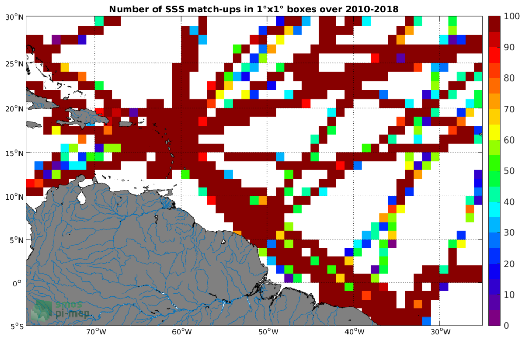
Figure 4: Number of SSS match-ups between TSG-GOSUD-Research-vessel SSS and the SMOS L3 v317 - 10 Days - 25 km (CATDS-CPDC) SSS product for the Amazon and Orinoco river plumes Pi-MEP region over 1°x1° boxes and for the full satellite product period.
