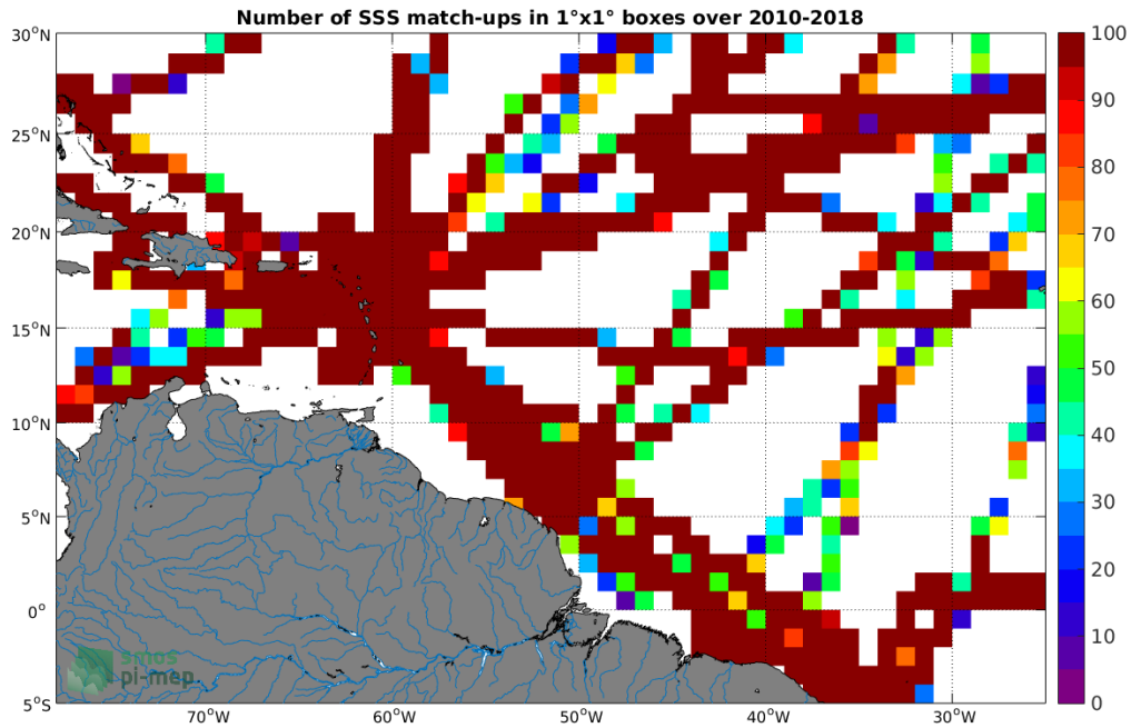
Figure 4: Number of SSS match-ups between TSG-GOSUD-Research-vessel SSS and the SMOS-L3-CATDS-CPDC-V317-10DAYS-25KM SSS product for the Amazon and Orinoco river plumes Pi-MEP region over 1°x1° boxes and for the full satellite product period.
