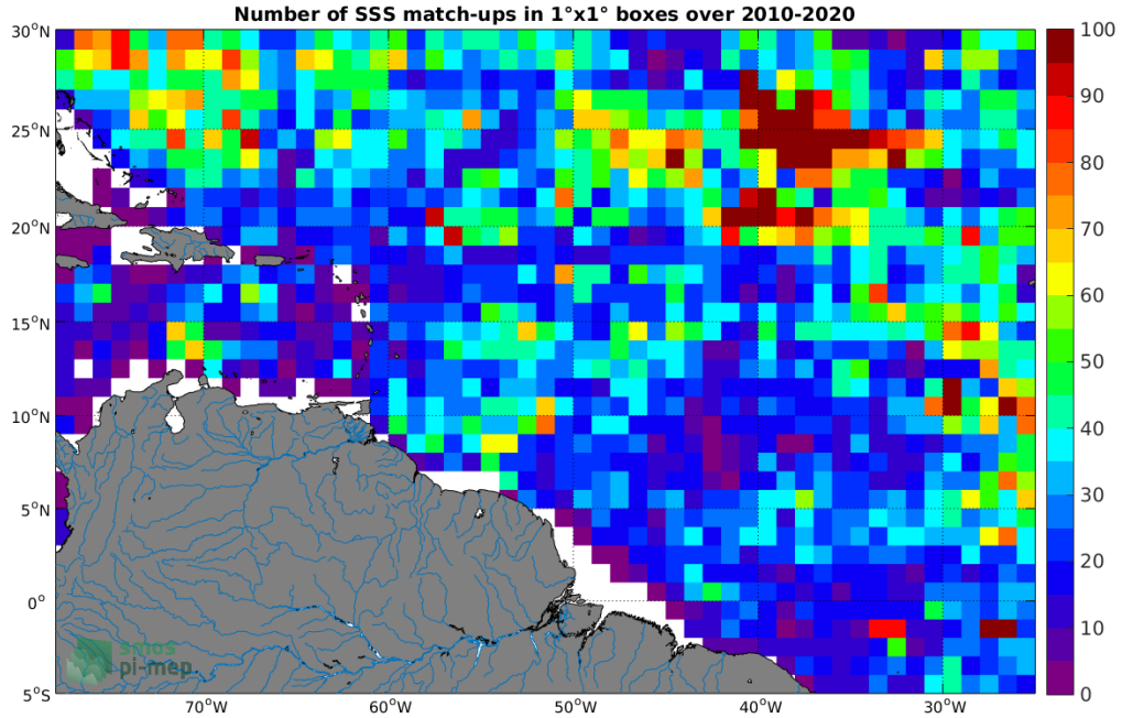
Figure 4: Number of SSS match-ups between Argo SSS and the SMOS SSS L3 v317 - 10 Days - 25 km (CATDS-CPDC) SSS product for the Amazon and Orinoco river plumes Pi-MEP region over 1°x1° boxes and for the full satellite product period.
