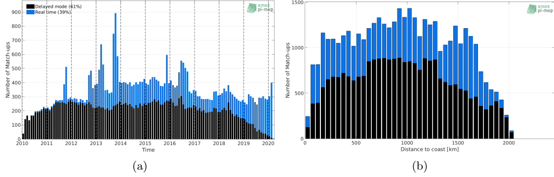
Figure 1: Number of match-ups between Argo and SMOS L3 v317 - 10 Days - 25 km (CATDS-CPDC) SSS as a function of time (a) and as function of the distance to coast (b) over the Amazon and Orinoco river plumes Pi-MEP region and for the full satellite product period.
