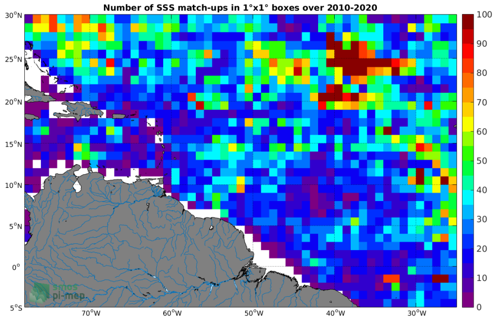
Figure 4: Number of SSS match-ups between Argo SSS and the SMOS L3 v317 - 10 Days - 25 km (CATDS-CPDC) SSS product for the Amazon and Orinoco river plumes Pi-MEP region over 1°x1° boxes and for the full satellite product period.
