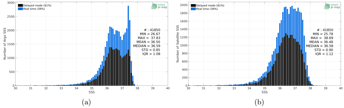
Figure 2: Histograms of SSS from Argo (a) and SMOS L3 v317 - 10 Days - 25 km (CATDS-CPDC) (b) considering all match-up pairs per bins of 0.1 over the Amazon and Orinoco river plumes Pi-MEP region and for the full satellite product period.
