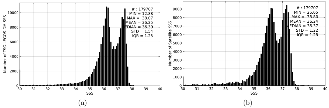
Figure 2: Histograms of SSS from TSG-LEGOS-DM (a) and SMOS-L3-CATDS-CPDC-V3-MONTHLY-25KM (b) considering all match-up pairs per bins of 0.1 over the Amazon and Orinoco river plumes Pi-MEP region and for the full satellite product period.
