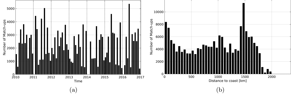
Figure 1: Number of match-ups between TSG-LEGOS-DM and SMOS-L3-CATDS-CPDC-V3-MONTHLY-25KM SSS as a function of time (a) and as function of the distance to coast (b) over the Amazon and Orinoco river plumes Pi-MEP region and for the full satellite product period.
