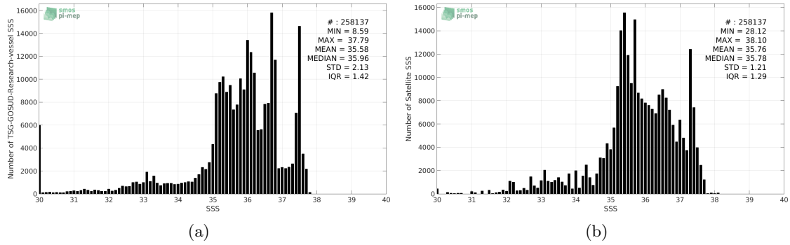
Figure 2: Histograms of SSS from TSG-GOSUD-Research-vessel (a) and SMOS-L3-CATDS-CPDC-V3-MONTHLY-25KM (b) considering all match-up pairs per bins of 0.1 over the Amazon and Orinoco river plumes Pi-MEP region and for the full satellite product period.
