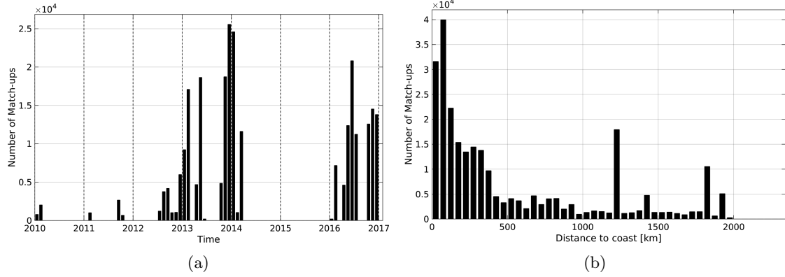
Figure 1: Number of match-ups between TSG-GOSUD-Research-vessel and SMOS-L3-CATDS-CPDC-V3-MONTHLY-25KM SSS as a function of time (a) and as function of the distance to coast (b) over the Amazon and Orinoco river plumes Pi-MEP region and for the full satellite product period.
