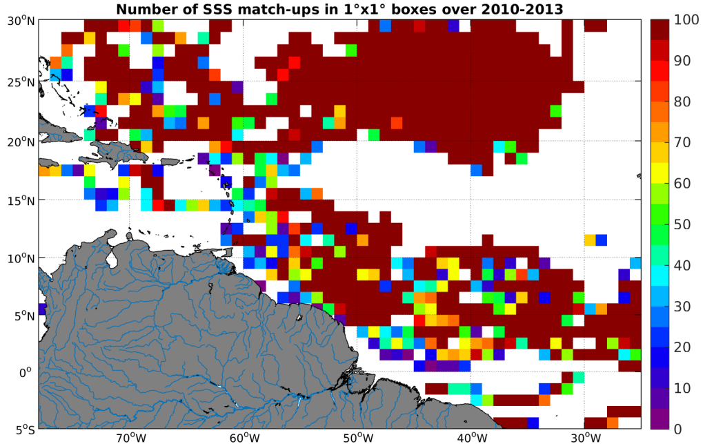
Figure 3: Number of SSS match-ups between Surface drifters SSS and the SMOS-L3-CATDS-CPDC-V3-MONTHLY-25KM SSS product for the Amazon and Orinoco river plumes Pi-MEP region over 1^\circ \times 1^\circ boxes and for the full satellite product period.
