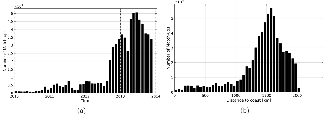
Figure 1: Number of match-ups between Surface drifters and SMOS-L3-CATDS-CPDC-V3-MONTHLY-25KM SSS as a function of time (a) and as function of the distance to coast (b) over the Amazon and Orinoco river plumes Pi-MEP region and for the full satellite product period.
