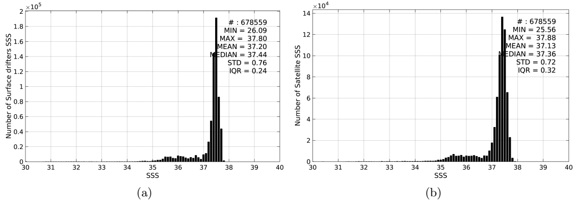
Figure 2: Histograms of SSS from Surface drifters (a) and SMOS-L3-CATDS-CPDC-V3-MONTHLY-25KM (b) considering all match-up pairs per bins of 0.1 over the Amazon and Orinoco river plumes Pi-MEP region and for the full satellite product period.
