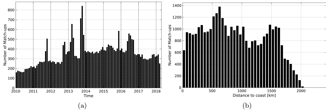
Figure 1: Number of match-ups between Argo and SMOS-L3-CATDS-CPDC-V3-MONTHLY-25KM SSS as a function of time (a) and as function of the distance to coast (b) over the Amazon and Orinoco river plumes Pi-MEP region and for the full satellite product period.
