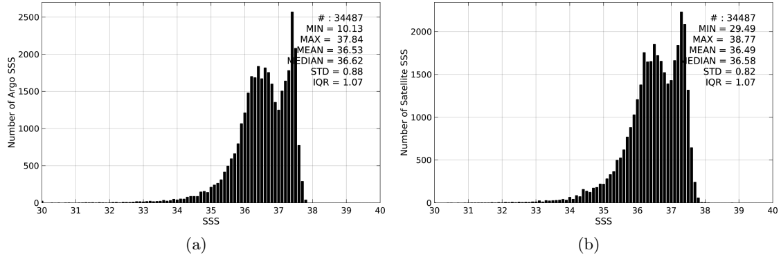
Figure 2: Histograms of SSS from Argo (a) and SMOS-L3-CATDS-CPDC-V3-MONTHLY-25KM (b) considering all match-up pairs per bins of 0.1 over the Amazon and Orinoco river plumes Pi-MEP region and for the full satellite product period.
