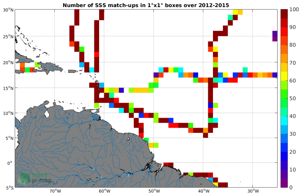
Figure 4: Number of SSS match-ups between TSG-GOSUD-Sailing-ship SSS and the SMOS-L3-CATDS-CPDC-V3-10DAYS-25KM SSS product for the Amazon and Orinoco river plumes Pi-MEP region over 1^\circ \times 1^\circ boxes and for the full satellite product period.
