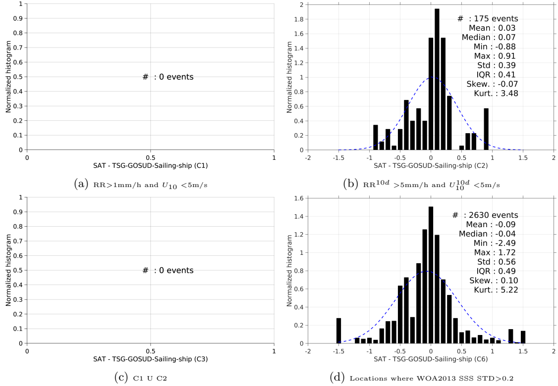
Figure 13: Normalized histogram of \Delta SSS (SMOS-L3-CATDS-CPDC-V3-10DAYS-25KM - TSG-GOSUD-Sailing-ship) for 6 different subdatasets corresponding to: RR > 1\text{mm/h} and U_{10} < 5\text{m/s} (a), RR^{10d} > 5\text{mm/h} and U_{10}^{10d} < 5\text{m/s} (b), C1 \cup C2 (c), Locations where WOA2013 SSS STD > 0.2 (d).
