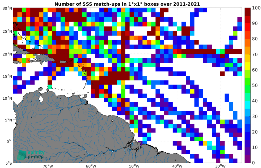
Figure 5: Number of SSS match-ups between TSG (SAMOS) SSS and the SMOS SSS L3 v2 - 9-Days (BEC) SSS product for the Amazon and Orinoco river plumes Pi-MEP region over 1^\circ \times 1^\circ boxes and for the full satellite product period.
