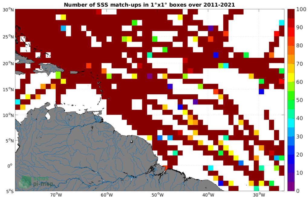
Figure 4: Number of SSS match-ups between TSG (SAMOS) SSS and the SMOS SSS L3 v2 - 9-Days (BEC) SSS product for the Amazon and Orinoco river plumes Pi-MEP region over 1^{\circ} \times 1^{\circ} boxes and for the full satellite product period.
