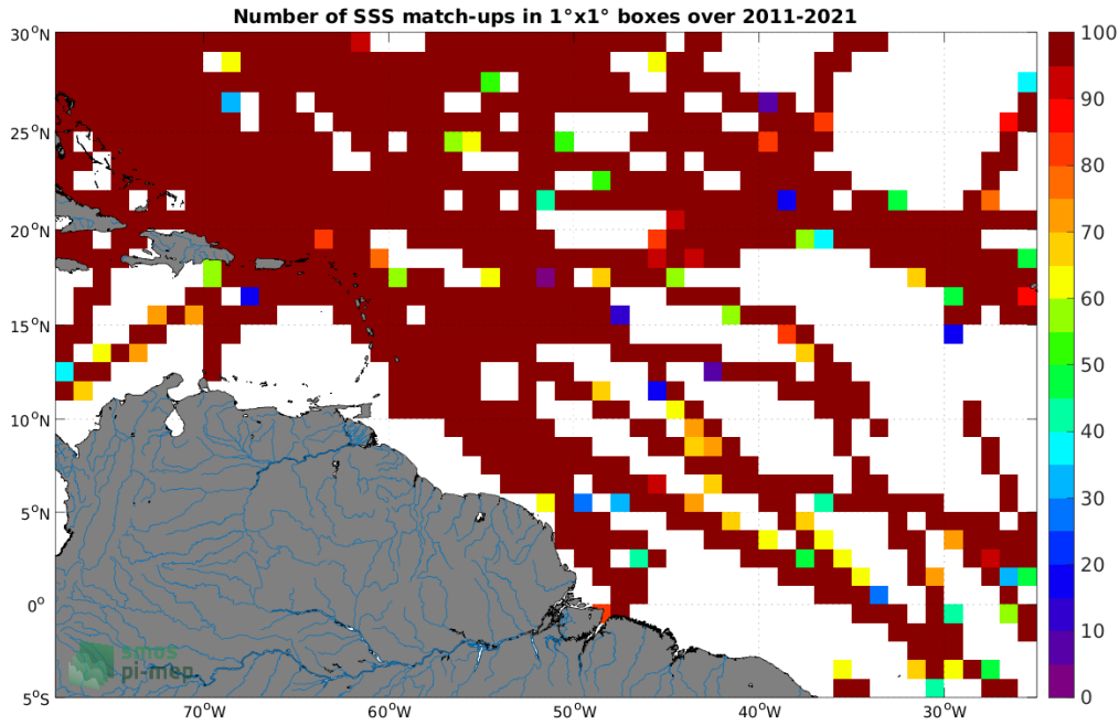
Figure 4: Number of SSS match-ups between TSG (SAMOS) SSS and the SMOS SSS L3 v2 - 9-Days (BEC) SSS product for the Amazon and Orinoco river plumes Pi-MEP region over 1^\circ \times 1^\circ boxes and for the full satellite product period.
