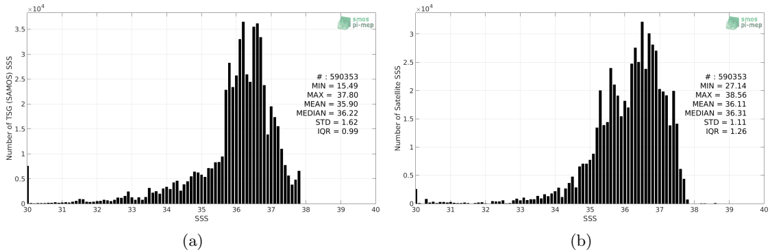
Figure 2: Histograms of SSS from TSG (SAMOS) (a) and SMOS L3 v2 - 9-Days (BEC) (b) considering all match-up pairs per bins of 0.1 over the Amazon and Orinoco river plumes Pi-MEP region and for the full satellite product period.
