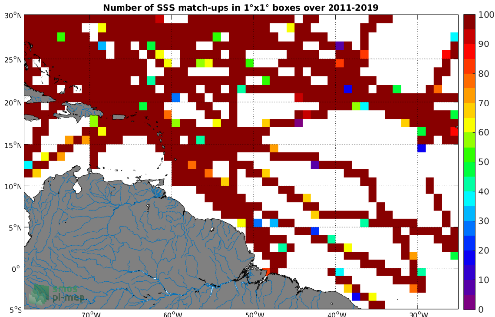
Figure 4: Number of SSS match-ups between TSG (SAMOS) SSS and the SMOS L3 v2 - 9-Days (BEC) SSS product for the Amazon and Orinoco river plumes Pi-MEP region over 1°x1° boxes and for the full satellite product period.
