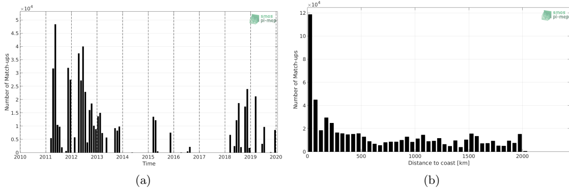
Figure 1: Number of match-ups between TSG (SAMOS) and SMOS L3 v2 - 9-Days (BEC) SSS as a function of time (a) and as function of the distance to coast (b) over the Amazon and Orinoco river plumes Pi-MEP region and for the full satellite product period.
