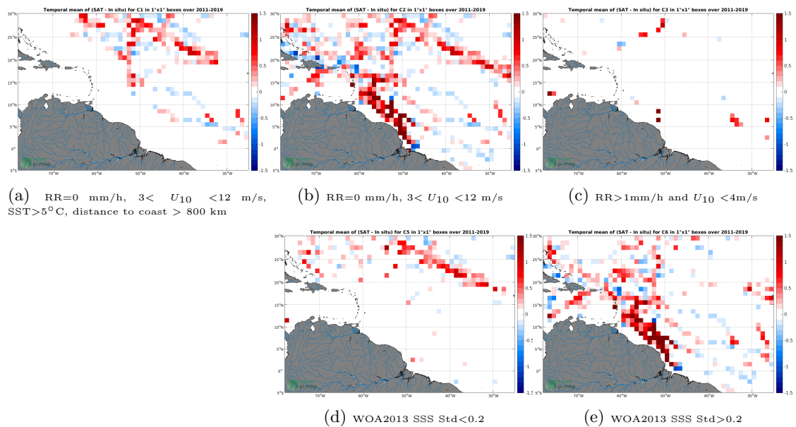
Figure 12: Temporal mean gridded over spatial boxes of size 1^\circ \times 1^\circ of \Delta SSS (SMOS L3 v2 - 9-Days (BEC) - TSG (SAMOS)) for 5 different subdatasets corresponding to: RR=0 mm/h, 3 < U_{10} < 12 m/s, SST > 5^\circ C , distance to coast > 800 km (a), RR=0 mm/h, 3 < U_{10} < 12 m/s (b), RR > 1 mm/h and U_{10} < 4 m/s (c), WOA2013 SSS Std < 0.2 (d), WOA2013 SSS Std > 0.2 (e).
