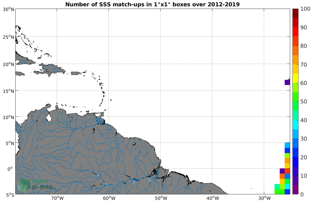
Figure 4: Number of SSS match-ups between TSG (Polarstern) SSS and the SMOS SSS L3 v2 - 9-Days (BEC) SSS product for the Amazon and Orinoco river plumes Pi-MEP region over 1°x1° boxes and for the full satellite product period.
