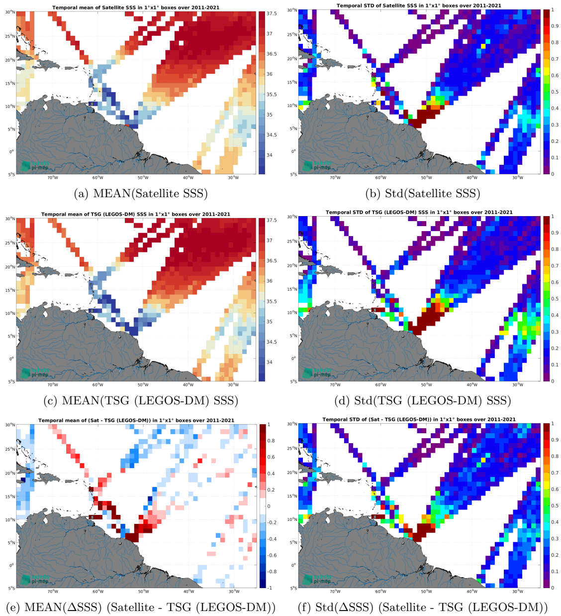
Figure 7: Temporal mean (left) and Std (right) of SSS from SMOS SSS L3 v2 - 9-Days (BEC) (top), TSG (LEGOS-DM) (middle), and of \Delta SSS (Satellite - TSG (LEGOS-DM)). Only match-up pairs are used to generate these maps.
