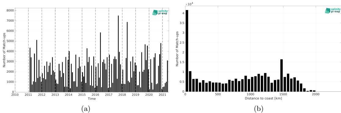
Figure 2: Number of match-ups between TSG (LEGOS-DM) and SMOS SSS L3 v2 - 9-Days (BEC) SSS as a function of time (a) and as function of the distance to coast (b) over the Amazon and Orinoco river plumes Pi-MEP region and for the full satellite product period.
