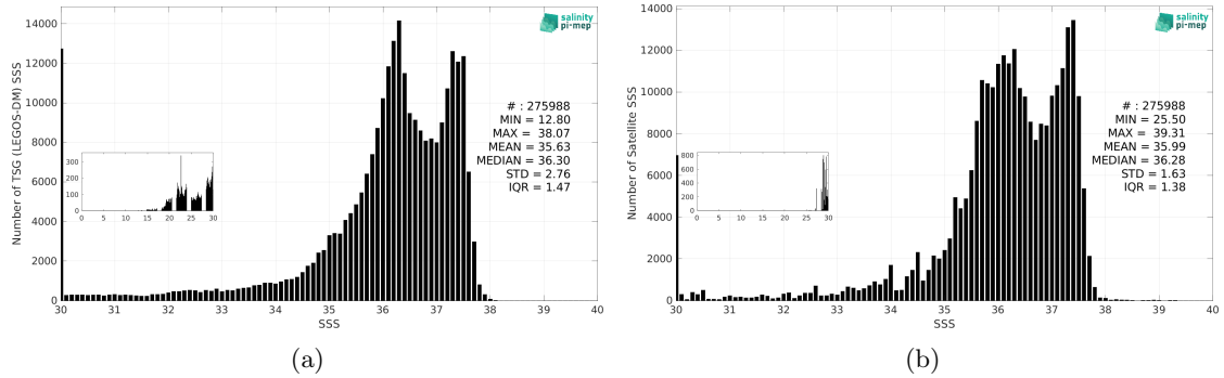
Figure 3: Histograms of SSS from TSG (LEGOS-DM) (a) and SMOS SSS L3 v2 - 9-Days (BEC) (b) considering all match-up pairs per bins of 0.1 over the Amazon and Orinoco river plumes Pi-MEP region and for the full satellite product period.
