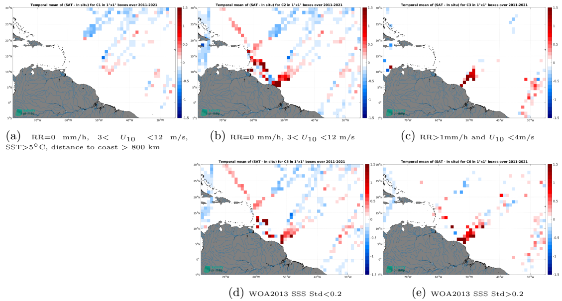
Figure 14: Temporal mean gridded over spatial boxes of size 1^\circ \times 1^\circ of \Delta SSS (SMOS SSS L3 v2 - 9-Days (BEC) - TSG (LEGOS-DM)) for 5 different subdatasets corresponding to:RR=0 mm/h, 3 < U_{10} < 12 m/s, SST>5°C, distance to coast > 800 km (a), RR=0 mm/h, 3 < U_{10} < 12 m/s (b), RR>1mm/h and U_{10} < 4 m/s (c), WOA2013 SSS Std<0.2 (d), WOA2013 SSS Std>0.2 (e).
