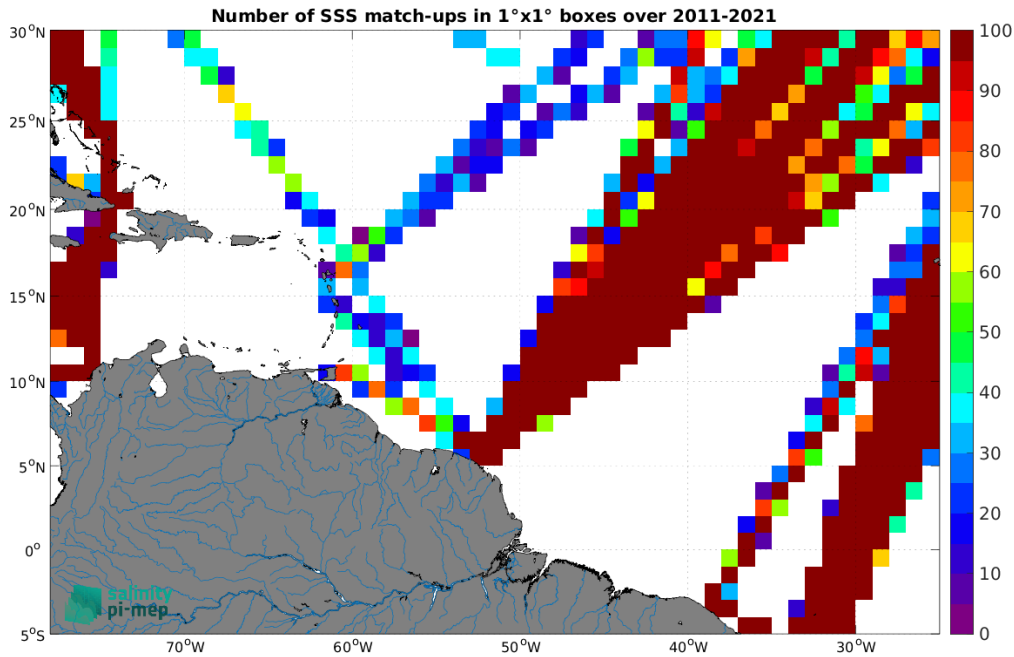
Figure 5: Number of SSS match-ups between TSG (LEGOS-DM) SSS and the SMOS SSS L3 v2 - 9-Days (BEC) SSS product for the Amazon and Orinoco river plumes Pi-MEP region over 1^\circ \times 1^\circ boxes and for the full satellite product period.
