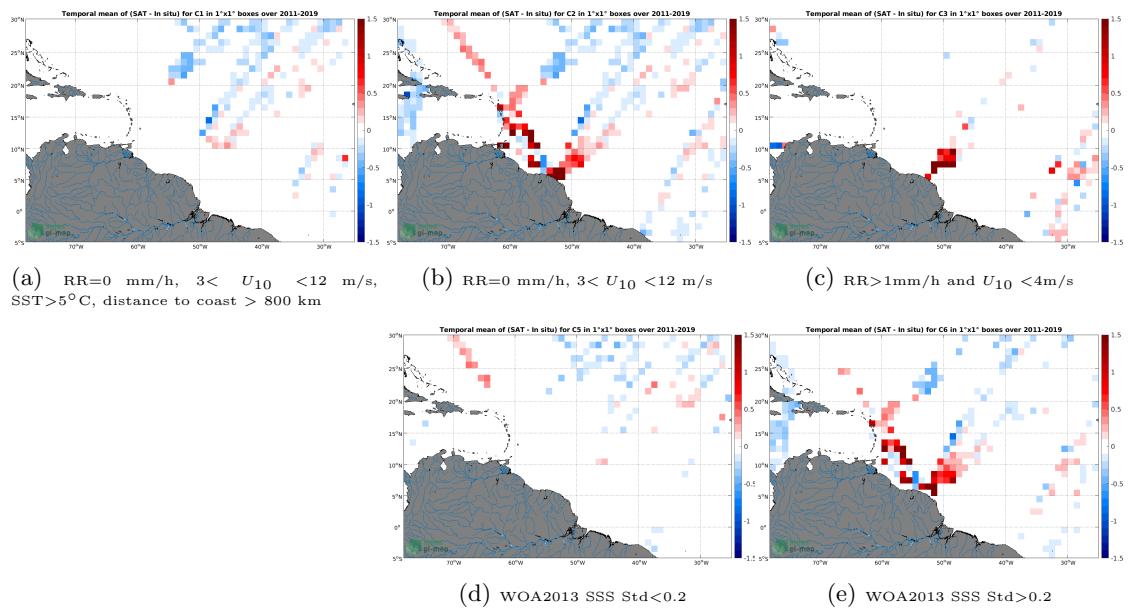
Figure 12: Temporal mean gridded over spatial boxes of size 1^\circ \times 1^\circ of \Delta SSS (SMOS SSS L3 v2 - 9-Days (BEC) - TSG (LEGOS-DM)) for 5 different subdatasets corresponding to: RR=0 mm/h, 3 < U_{10} < 12 m/s, SST > 5°C, distance to coast > 800 km (a), RR=0 mm/h, 3 < U_{10} < 12 m/s (b), RR > 1mm/h and U_{10} < 4 m/s (c), WOA2013 SSS Std < 0.2 (d), WOA2013 SSS Std > 0.2 (e).
