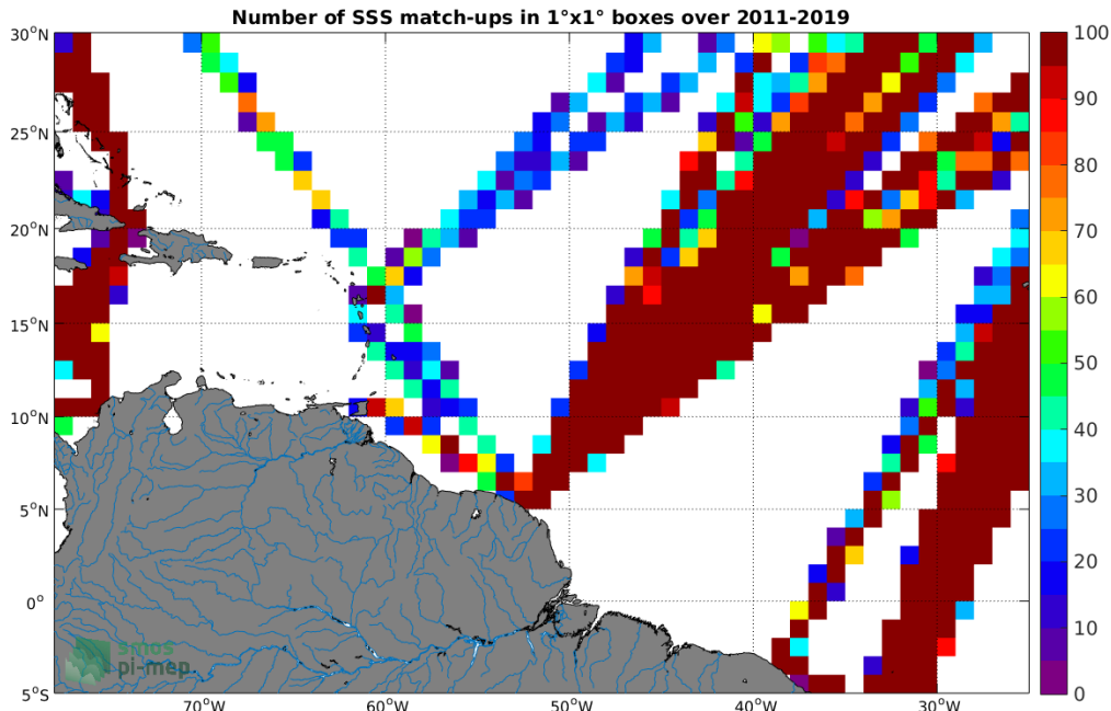
Figure 4: Number of SSS match-ups between TSG (LEGOS-DM) SSS and the SMOS L3 v2 - 9-Days (BEC) SSS product for the Amazon and Orinoco river plumes Pi-MEP region over 1°x1° boxes and for the full satellite product period.
