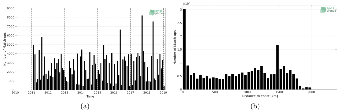
Figure 1: Number of match-ups between TSG (LEGOS-DM) and SMOS L3 v2 - 9-Days (BEC) SSS as a function of time (a) and as function of the distance to coast (b) over the Amazon and Orinoco river plumes Pi-MEP region and for the full satellite product period.
