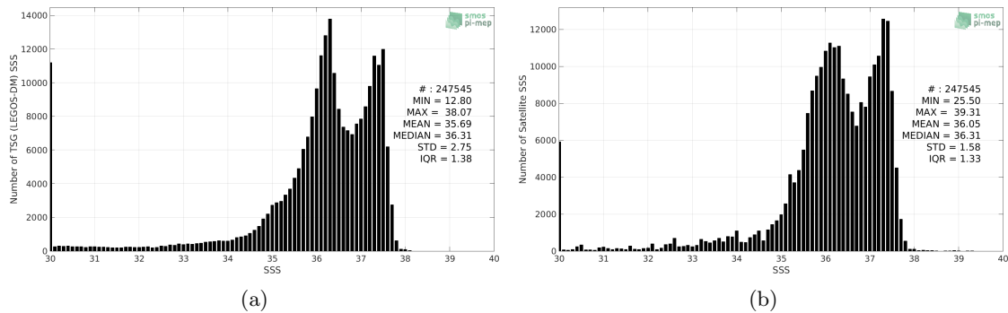
Figure 2: Histograms of SSS from TSG (LEGOS-DM) (a) and SMOS L3 v2 - 9-Days (BEC) (b) considering all match-up pairs per bins of 0.1 over the Amazon and Orinoco river plumes Pi-MEP region and for the full satellite product period.
